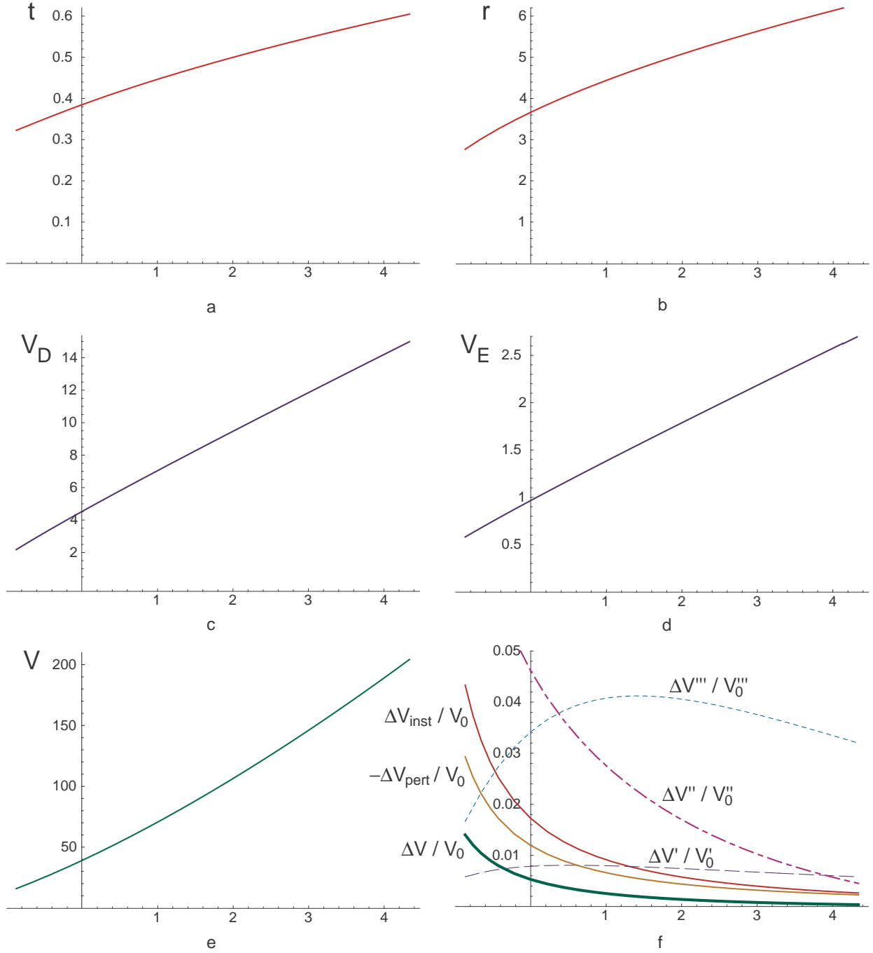
Fig. 19: Numerical results for critical point moduli as a function of the flux superpotential |\widetilde{W}_0| . The x -axis shows everywhere -\log_{10} |\widetilde{W}_0| and the y -axis in (a): t , (b): r , (c): V_D , (d): V_E and (e): V , as defined in (6.16). Finally (f) shows the estimated relative size of perturbative and instanton corrections to V and its derivatives \partial_t^k V , k = 1, 2, 3 , for g_s \sim 1/4 .
