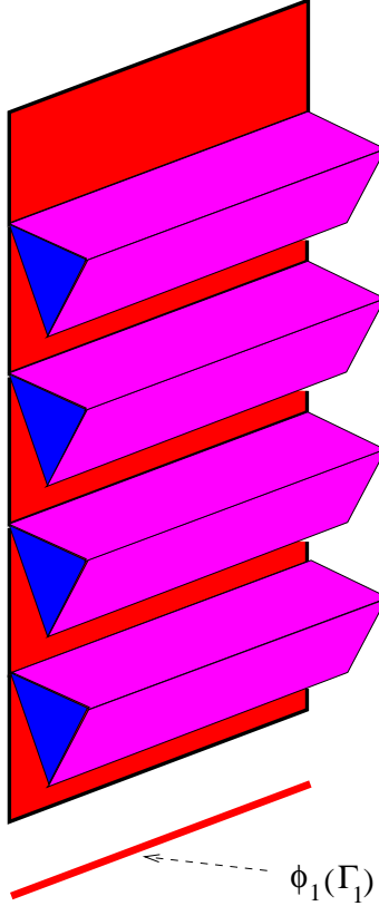
Fig. 16: The surface in Z_2 over \phi_1(\Gamma_1) after the first contraction, following \phi_1 .
