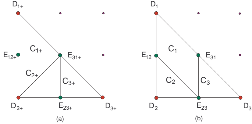
Fig. 2: Fan for (a) asymmetric and (b) symmetric resolution of \mathbb{C}^3/\mathbb{Z}_2 \times \mathbb{Z}_2 .
