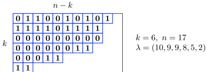
FIGURE 2. A J-diagram (\lambda, D)_{k,n}
