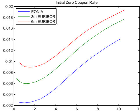
FIGURE 8.8. Zero coupon rates, EUR market, 27 May 2013.
