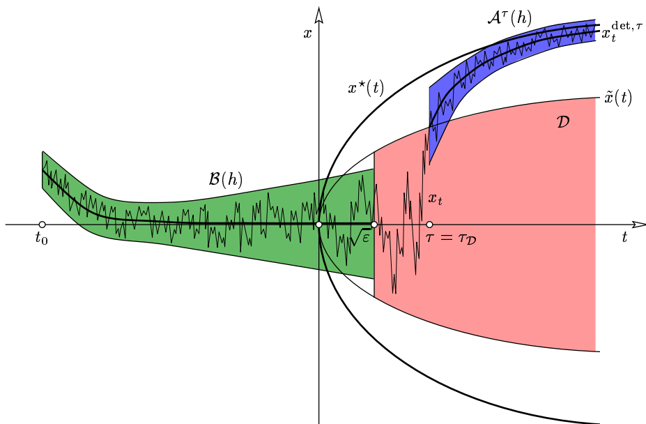
FIGURE 2. A typical path x_t of the stochastic differential equation (1.5) near a pitchfork bifurcation. We prove that with probability exponentially close to 1, the path has the following behaviour. For t_0 \leq t \leq \sqrt{\varepsilon} , it stays in a strip \mathcal{B}(h) constructed around the deterministic solution with the same initial condition. After t = \sqrt{\varepsilon} , it leaves the domain \mathcal{D} at a random time \tau = \tau_{\mathcal{D}} , which is typically of the order \sqrt{\varepsilon|\log \sigma|} . Then it stays (up to times of order 1 at least) in a strip \mathcal{A}^\tau(h) constructed around the deterministic solution x_t^{\text{det}, \tau} starting at time \tau on the boundary of \mathcal{D} . The widths of \mathcal{B}(h) and \mathcal{A}^\tau(h) are proportional to a parameter h satisfying \sigma \ll h \ll \sqrt{\varepsilon} .
