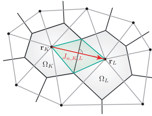
Fig. 3. Delaunay triangulation and construction of Voronoi cells. The red arrow indicates the discrete current J_{n,K,L} between two neighboring control volumes \Omega_K and \Omega_L . The green area is the bi-hyperpyramid with height \|\mathbf{r}_L - \mathbf{r}_K\| and internal face |\partial\Omega_L \cap \partial\Omega_K| .
