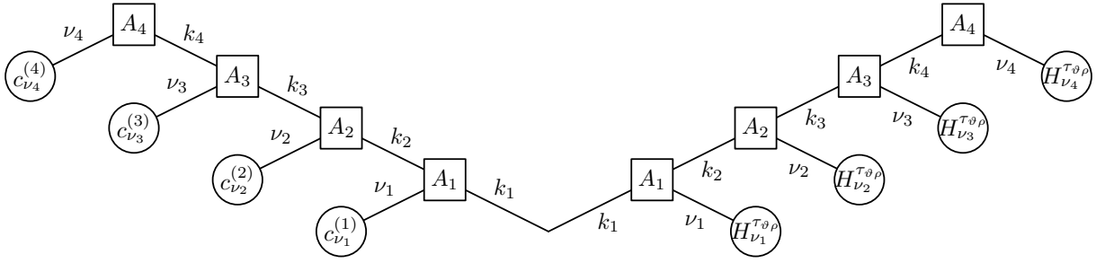
FIGURE 1. A coefficient splitting for L = 4 .
