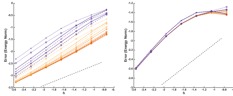
Figure 4: Example I: Error in the mesh dependent norm (15) against the mesh size (in double logarithmic scale), for the cases (\mu_{\text{eff}}, \sigma) = (1, 1) (left) and (\mu_{\text{eff}}, \sigma) = (0.001, 10) (right). A dashed line with slope equal to one is also shown.
