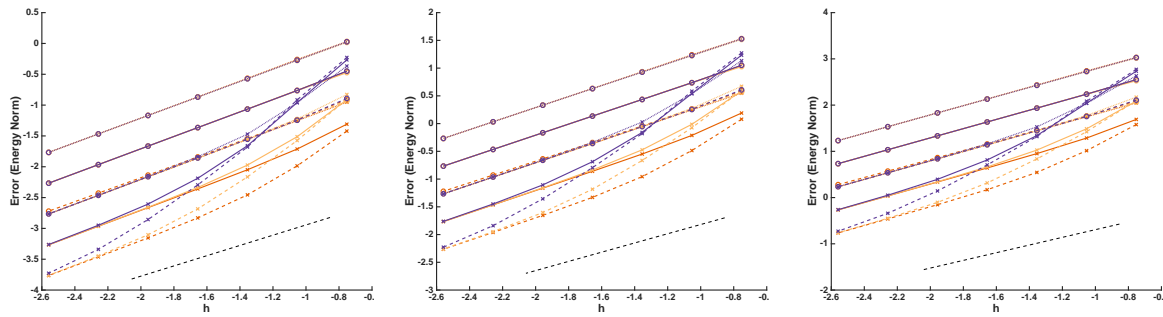
Figure 7: Example II: Error in the mesh dependent norm (15) against the mesh size (in double logarithmic scale), for the cases \sigma = 0.001 (left), \sigma = 1 (center), and \sigma = 1000 (right). The dashed line visualizes a slope equal to 1.
