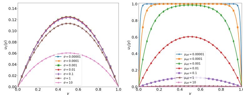
Figure 3: Example I: The function u_1(y) defined in (61b) with fixed \mu_{\text{eff}} = 1 for different values of \sigma (left) and with fixed \sigma = 1 for different values of \mu_{\text{eff}} (right).
