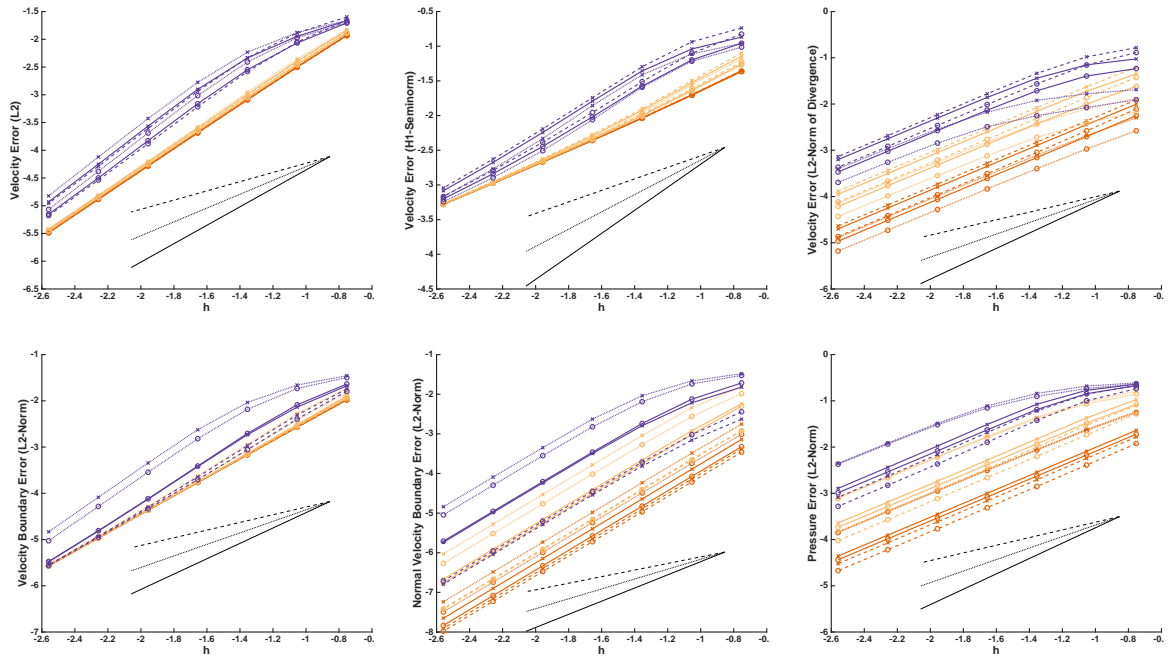
Figure 5: Example I: Velocity and pressure errors against the mesh size (in double logarithmic scale), for the case (\mu_{\text{eff}}, \sigma) = (1, 1) . The lines with slope equal to 1 (dashed), \frac{3}{2} (dotted) and 2 (solid) are also shown.
