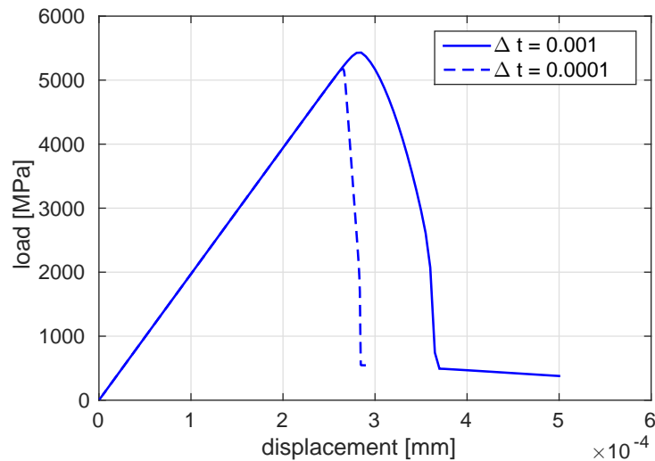
Figure 11: Load-deflection curve
