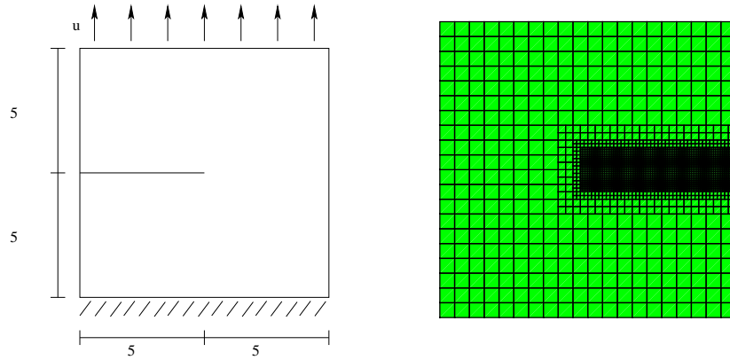
Figure 3: Boundary conditions (left) of a mode-I-tension test and the related mesh based on a hierarchical refinement strategy (right)
