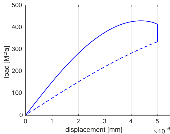
Figure 4: Load-deflection curve of the mode-I-tension test under loading and unloading at different time steps.
