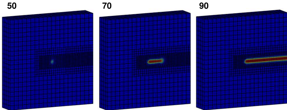
Figure 10: Phase-field snapshots of the mode-I-tension test at different times.
