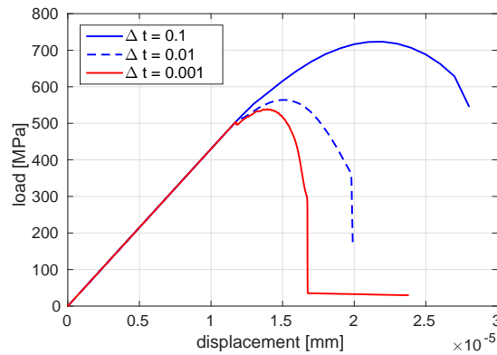
Figure 8: Load-deflection curves for different time step sizes
