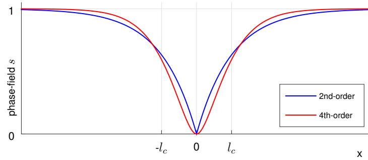
Figure 1: Uniaxial model with a crack at x = 0 and with a continuous phase-field s \in [0, 1] ; phase-field approximation for a second order and a fourth order approximation of the crack density function \gamma .
