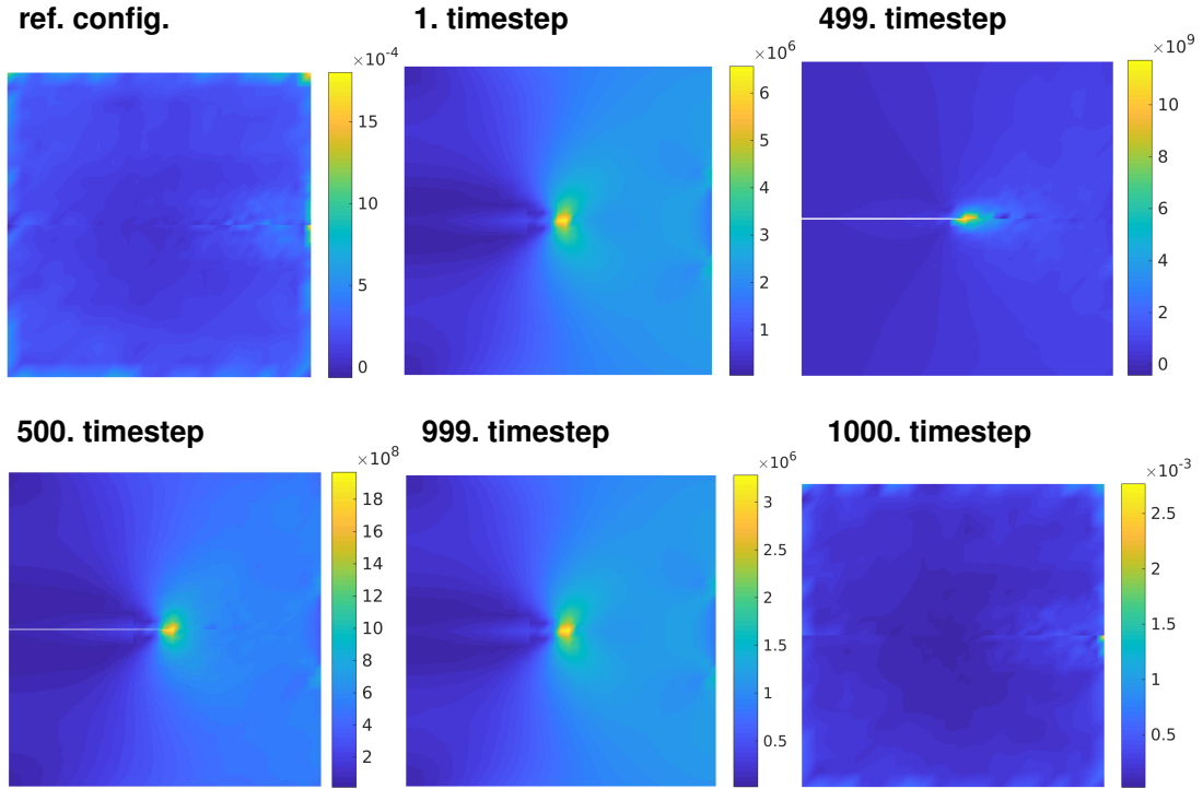
Figure 5: Von Mises stresses of the mode-I-tension test under loading and unloading at different time steps.
