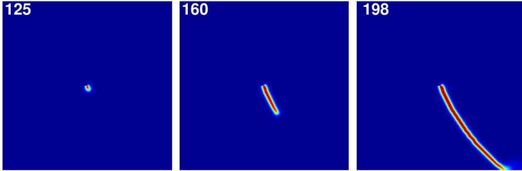
Figure 7: Phase-field snapshots of the mode-II-shear test at different times.
