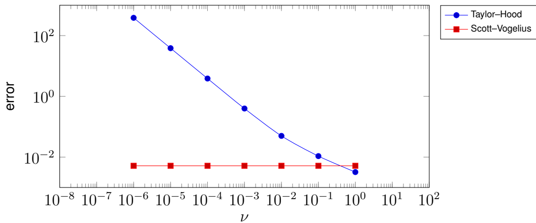
Figure 1: Best approximation error (13) of the Taylor-Hood and Scott-Vogelius finite element methods versus \nu on a fixed unstructured mesh with 201 vertices in Example 4.2.
