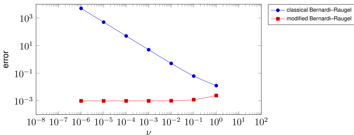
Figure 2: Best approximation error (13) of the classical and modified Bernardi–Raugel finite element method versus \nu on a fixed unstructured mesh with 277 vertices in Example 7.2.
