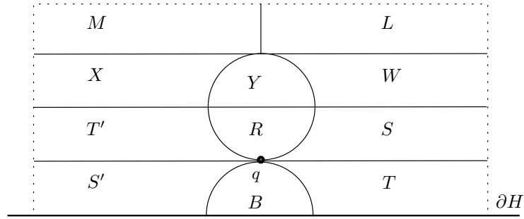
FIGURE A.2. Formula (??) evaluated at q = (0, \rho) .
