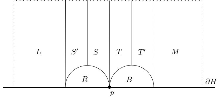
FIGURE A.1. Formula (??) evaluated at p = (-\rho, 0) .
