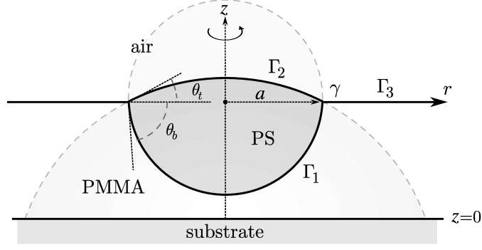
Figure 4: Sketch of a axisymmetric liquid lens in equilibrium with \Gamma_1, \Gamma_2, \Gamma_3 being the PS/PMMA, PS/air, PMMA/air interface respectively and \gamma the triple-junction. Each interface \Gamma_i has the surface tension \sigma_i . The radius of the lens is a and the contact angles are \theta_t, \theta_b (top, bottom). Furthermore for planar axisymmetric droplets we have \mathbf{n}_{\Gamma_1} = -\mathbf{e}_r \cos \theta_b - \mathbf{e}_z \sin \theta_b , \mathbf{n}_{\Gamma_2} = -\mathbf{e}_r \cos \theta_t + \mathbf{e}_z \sin \theta_t , \mathbf{n}_{\Gamma_3} = \mathbf{e}_r .
