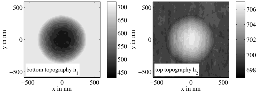
Figure 3: Measured equilibrium drop profile as determined by AFM. The height scales in nanometers are shown to the right of each panel. ( left ) bottom profile h_1 and ( right ) top profile h_2 .
