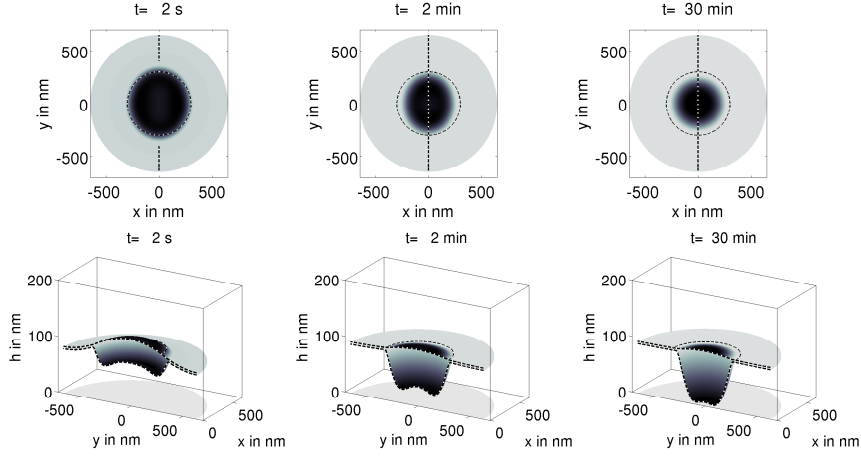
Figure 7: Numerical solutions of the 2d thin-film equation with nonsymmetric initial data and h_* = 1/5 and other parameters as before at t = 2 sec, 2 min, 30 min ( top ) top view ( bottom ) 3d view showing a quick evolution into a nearly axisymmetric state followed by an evolution where h_1 \rightarrow 0 .
