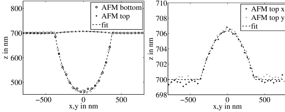
Figure 5: ( left ) Top and bottom AFM topography of an equilibrium droplet. Two cross sections cut perpendicular through the droplet in x -direction (dark symbols) and y -direction (light symbols) are shown together with the fit using eq. (5) (dashed line); ( right ) close-up of the top AFM topography including fit function.
