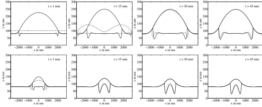
Figure 8: Numerical simulation of droplet formation and equilibration for two PS volumes and different initial configurations at different times. (top) r_0 = 32L, h = H and r_0 = 16L, h = 4H and (bottom) r_0 = 8L, h = H and r_0 = 4L, h = 4H ( H = 20 nm, L = 133 nm)
