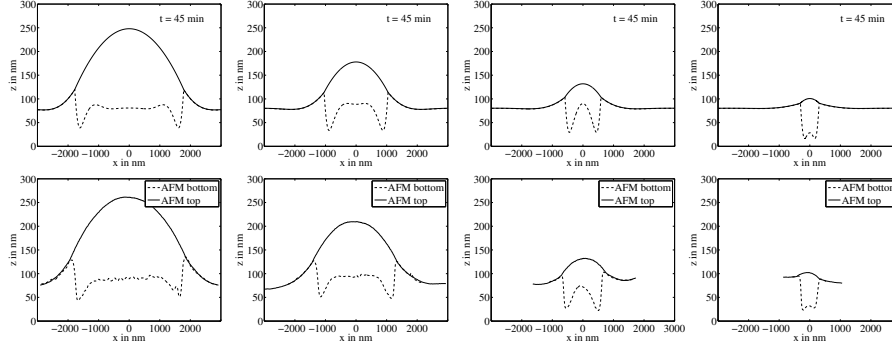
Figure 9: PS( 10k ) droplets on PMMA( 10k ) substrates at T = 140 °C after dewetting a sample for t = 45 min. The initially flat PMMA and PS layers had a thickness of h_1 = 80 nm and h_2 - h_1 = 20 nm, respectively. ( upper column ) simulations and ( lower column ) AFM measurements of similar volumes.
