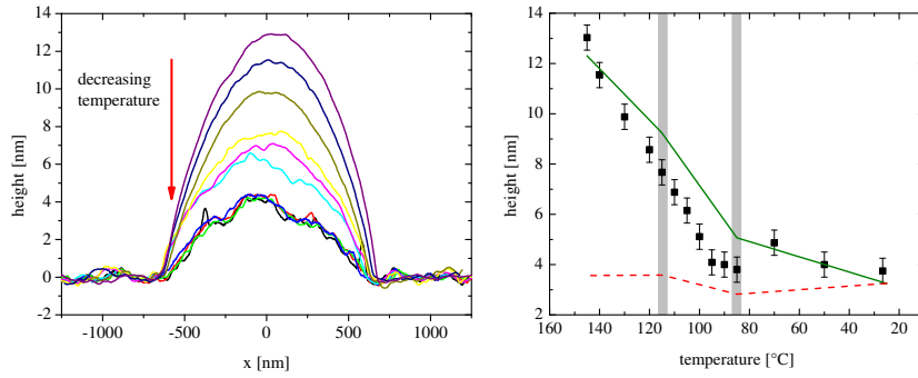
Figure 2: (left) Cross sections of the same polystyrene droplet imaged in situ by AFM while cooling the sample from 145 °C to 30 °C. The entire duration of this cooling cycle was about 70 minutes. (right) Temperature dependent height of the droplet as obtained from AFM data with glass transition temperatures of PS and PMMA are indicated. The solid line shows the expected height change based on thermal expansion polymers when assuming a constant width of the droplet. The dashed line denotes a similar model calculating assuming just the linear expansion coefficients.
