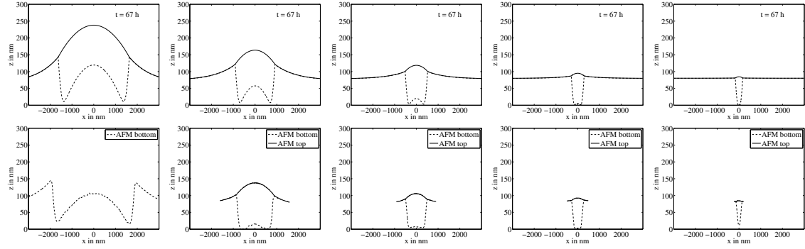
Figure 10: PS(10k) droplets on PMMA(10k) substrates at T = 140 °C after dewetting a sample for t = 67 h. The initially flat PMMA and PS layers had a thickness of h_1 = 80 nm and h_2 - h_1 = 20 nm, respectively. ( upper column ) simulations and ( lower column ) AFM measurements of similar volumes.
