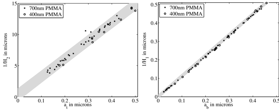
Figure 6: (top) Curvature of the top spherical caps and (bottom) curvature of bottom spherical caps as a function of droplet radius a measured from equilibrium droplets on 400 nm thick PMMA substrates (circles) and 700 nm thick PMMA substrates (crosses) with linear fit (shaded area 95% confidence interval) gives H_1^{-1} = (1.11 \pm 0.02)a_b and H_2^{-1} = (29 \pm 1)a_t and corresponding contact angles \theta_b = (64 \pm 2)^\circ and \theta_t = (1.98 \pm 0.07)^\circ .
