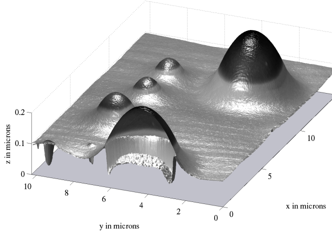
Figure 1: Composition of AFM top and bottom topographies after dewetting at T = 140\text{ }^{\circ}\text{C} for 45 min. Initial top layer thickness 80 nm PMMA and bottom layer thickness 20 nm PS layer lead to isolated droplets, which are not yet in equilibrium
