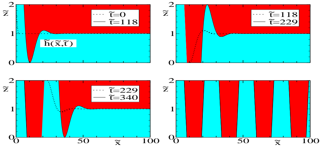
Figure 4: Numerical simulations using the thin film approximation (5.2a), starting from an initial hole near x = 0 with the B-rich phase (blue, light) penetrating the A-rich phase (red, dark). Shown is the situation after the first, second, third and many rupture events, respectively. Results are given in terms of the rescaled variables \tilde{x} = \theta x and \tilde{t} = (\varepsilon d \theta^4 / 3) t .
