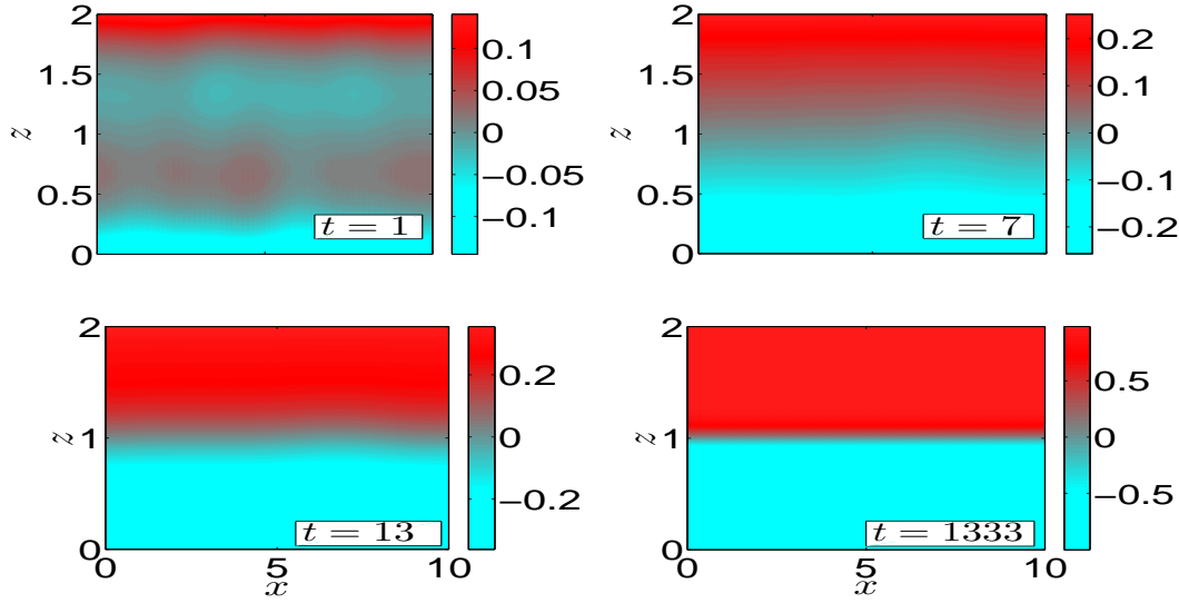
Figure 3: Phase-field simulations showing that a bilayer can be produced from a noisy initial condition if the temperature of the system is slowly cooled from the critical value and the substrates have a small amount of surface energy. See text for details.
