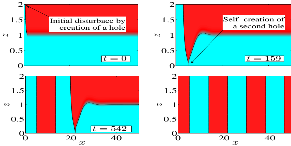
Figure 1: In a geometrically confined phase-field model with coordinate x that extend indefinitely in a direction parallel to two substrates at z = 0, d , a topological transformation in a bilayer of two phases is induced by the creation of a single hole (a) in the upper layer. Under the correct conditions, this initial hole can generate a second hole in the lower layer (b). This process repeats itself and triggers a cascade of hole generation (c) resulting into the creation of a periodic array of stripes (The contour line represents \phi = 0 in the phase-field model and the system is symmetric about x = 0 ; see text for details).
