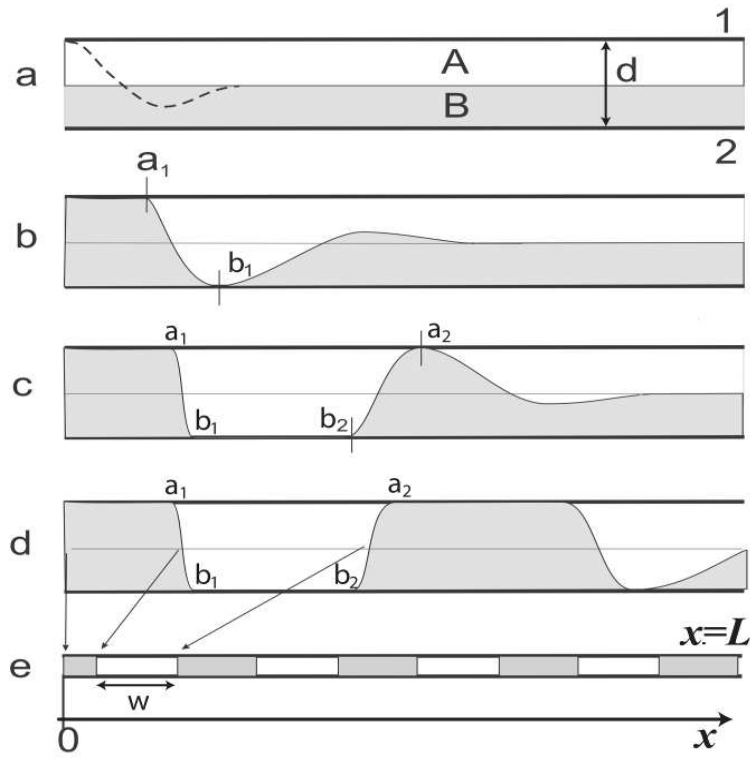
Figure 2: Configurations of interfaces between immiscible materials A and B during the topological transformation. The domains are symmetric with respect to x = 0 . Explanations are given in the text.
