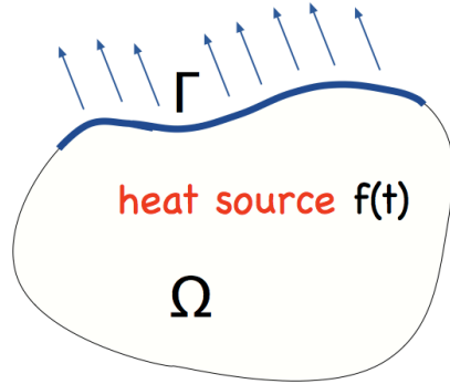
FIG. 1.1. Boundary control of a time dependent heat source.
