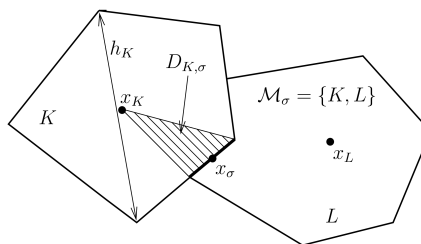
FIGURE 1. Notations for two neighboring control volumes in the case d = 2
