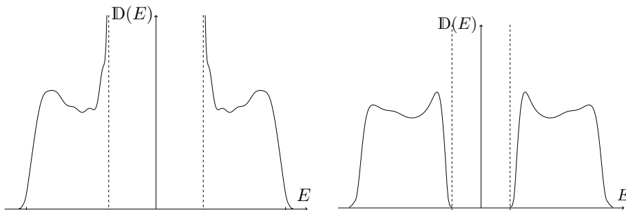
FIGURE 1. Comparison of the density of states of a random block operator \mathbb{H} without (left) and with (right) randomness in the off-diagonal blocks B . The singularities at the inner band edges are smoothed out by the randomness in B .
