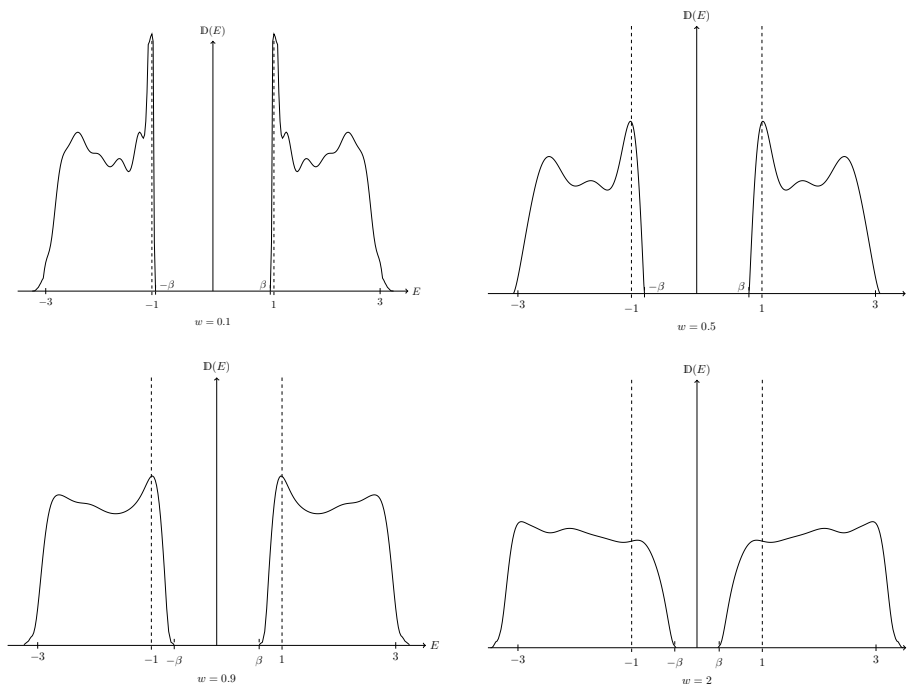
FIGURE 3. Assuming b_\omega(j) = 1 + w\tilde{b}_\omega(j) with \tilde{b}_\omega(j) distributed uniformly in the interval [-0.5, 0.5] we display the dependence of the density of states on the disorder parameter w . (Assumption (B) of Theorem 5.1 is satisfied for w = 0.1, 0.5, 0.9 ).
