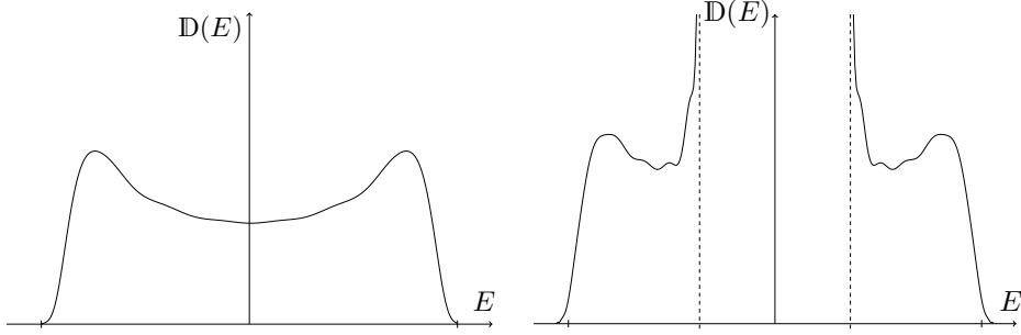
FIGURE 2. Comparison of the density of states of a random block operator \mathbb{H} with B = 0 (left) and B = \beta 1 (right).
