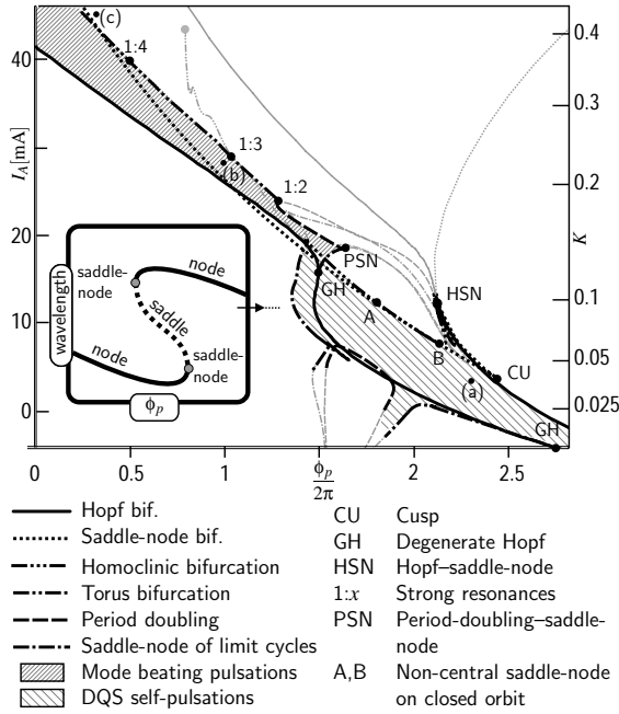
Figure 4: Bifurcation curves and islands of stable self-pulsations of the simplified two-mode model in the parameter plane (\phi_P, I_A) . The shaded islands indicate stable DQS and MB self-pulsations. Parameter as in the Table except \bar{g} = 0, \varepsilon = 0, \alpha_H = -4 . Furthermore \alpha_P is fixed to 20 \text{ cm}^{-1} , LSHB and thermal detuning are neglected. Inset: wavelength of stationary states vs. phase shift \phi_P schematically illustrating the double-fold structure above the cusp. The right-hand scale is the feedback strength K at the lower Hopf bifurcation.
