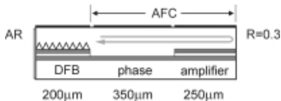
Figure 1: Schematics of the AFL used in this study. The combination of separate phase and amplifier sections allows for an independent phase and amplitude control of the feedback. AR: anti-reflection coated, R: facet power reflectivity.
