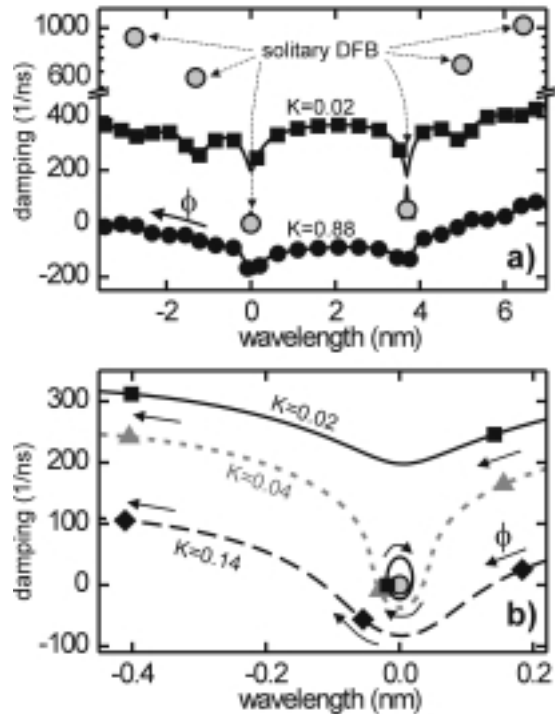
Figure 2: Spectrum of optical modes of an AFL. a) overview. b) environment of the lasing mode. Bullets: solitary laser ( K=0 ). Full symbols: K = 0.02, 0.04, 0.14 , and 0.88 , calculated under the following \varepsilon = 0 , no LSHB, feedback phase fixed. Lines: locations of modes for all possible feedback phases \phi . Arrows: direction of increasing \phi . After one phase period, each mode replaces its formerly next neighbor on the same line.
