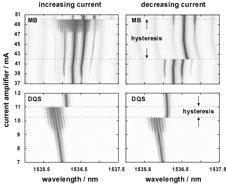
Figure 10: Comparison of optical spectra for increasing (left) and decreasing amplifier current (right) for the DQS and MB ranges indicated in Fig. 7 ( I_P=8 mA). The optical intensity is encoded in logarithmic grey scale.
