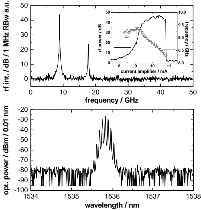
Figure 8: Power (upper panel) and optical (lower panel) spectrum ( I_{DFB}=70 mA, I_P=8 mA, I_A=9 mA). Inset: evolution of the primary peak of the power spectrum with increasing amplifier current I_A . Solid line: peak height, circles: frequency. Note the log-scale.
