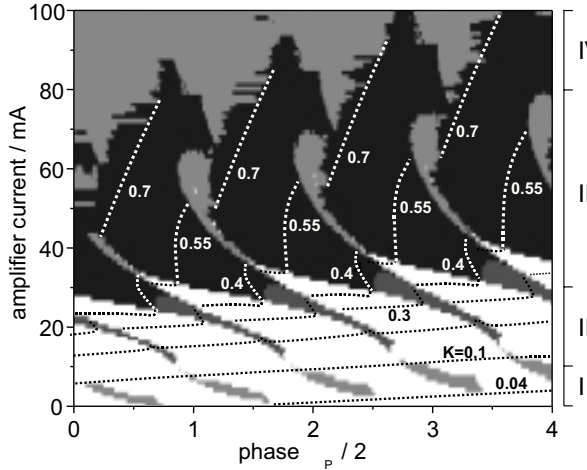
Figure 3: Calculated areas of self-pulsations in the plane spanned by the two parameters \phi_P and I_A . The DFB injection level was fixed to I_{\text{DFB}} = 70 mA, the damping in the phase section is increased by 5/\text{cm} per 2\pi . White areas correspond to cw output. Different levels of grey indicate non-stationary output with frequencies f (main peak of power spectrum) in the following ranges: f < 15 GHz (light), 15 \text{ GHz} < f < 30 GHz (dark), and f > 30 GHz (black). Dotted lines represent curves of constant K (averaged over one pulsation period in the self-pulsation areas).
