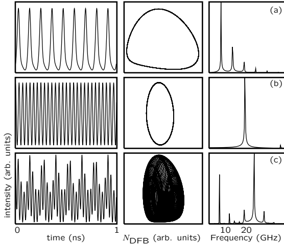
Figure 5: Dynamics in the points labeled (a) to (c) of the bifurcation diagram in Fig. 4. (a) typical low-frequency self-pulsation, (b) MB self-pulsation, (c) beyond the torus-bifurcation. Left column: output power versus time, middle column: projection of the phase space trajectory onto the plane of output power versus DFB carrier density, right column: power spectrum.
