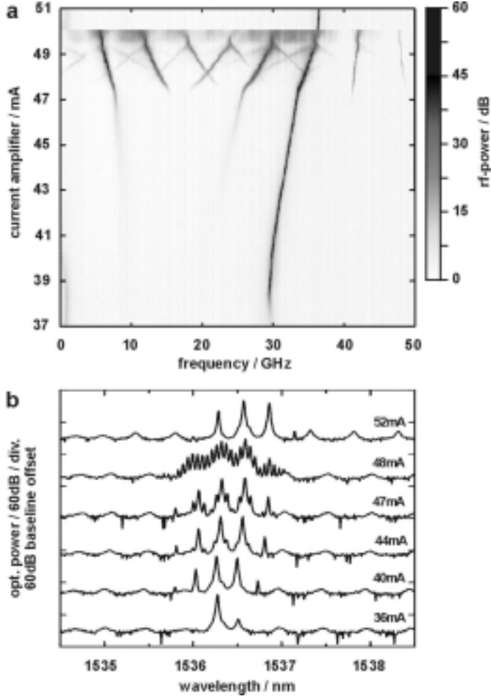
Figure 9: Characteristic spectra at high amplifier currents ( I_{DFB}=70 mA, I_P=8 mA). Panel a: power spectrum for I_A from 37 to 51 mA. The logarithmic grey scale codes the spectral intensity as denoted on the right-hand side. Panel b: log-scale optical spectra at selected points of panel a. Pure MB pulsation appears below I_A=47 mA, whereas the more complex spectral features above this amplifier current are due to the interaction between the relaxation oscillations and MB pulsations.
