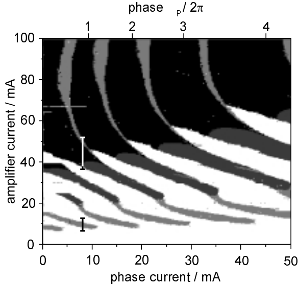
Figure 7: Areas of self-pulsations in the plane of phase and amplifier current. DFB current is fixed at 70 mA. For comparison with the numerical results, \phi_P is given at the top axis. The grey scale is the same as in Fig. 3. Only the frequency component with highest intensity is indicated. The vertical bars mark regions, where more details are presented in the subsequent figures.
