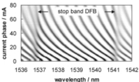
Figure 6: ASE measured at the amplifier facet with the DFB section pumped at transparency. The cavity between end-facet and DFB grating allows for a verification of the phase shift in the passive section. The excess loss by free carrier injection causes the damping of the ASE modulation with increasing current.
