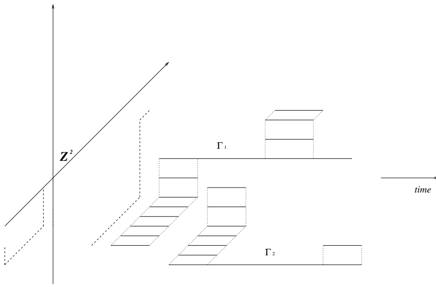
Figure 2: Two aggregates \Gamma_1 and \Gamma_2 having disjoint supports
