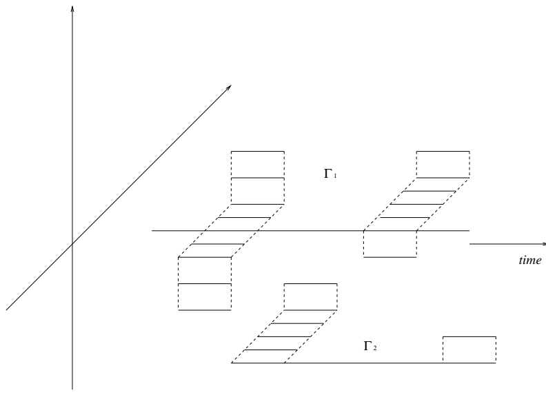
Figure 1: Two non-intersecting aggregates \Gamma_1 and \Gamma_2
