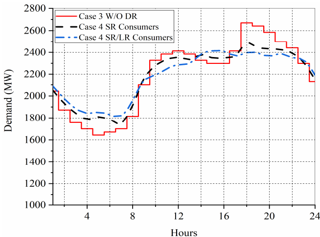
Fig. 6. Consumption profile for case 3 and case 4
