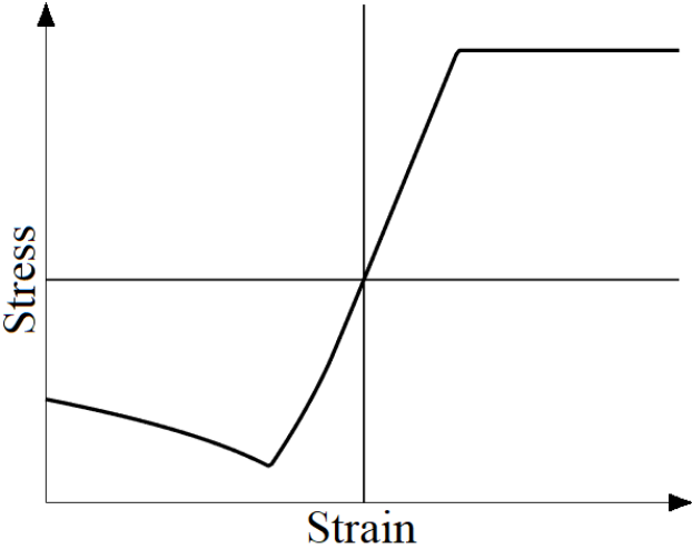
Figure 4. A schematic LSE curve with consideration of element buckling during compression.
