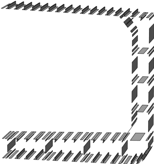
Figure 17. Example of discretization of a cross section in the Smith method models.
