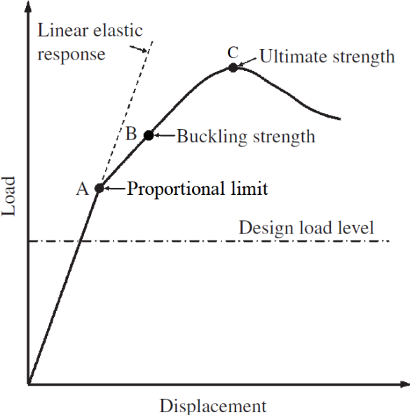
Figure 3. ULS behaviour of structures.
