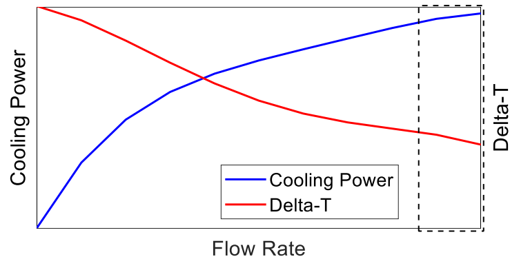
Figure 10: Illustration of saturation zone (area marked with dashed lines) for an increased cooling power, increased chilled water flow and with decreasing delta-T.
