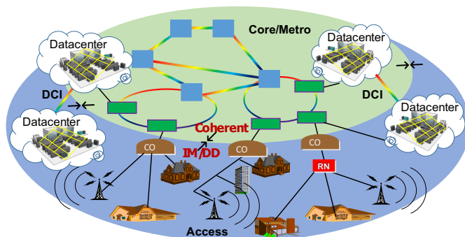
Fig. 1. A typical core, metro and access network scenario, including the metro-edge and intra-/inter-datacenter links, where the high-speed IM/DD links are required. CO: center office; RN: remote node; DCI: datacenter interconnects.
