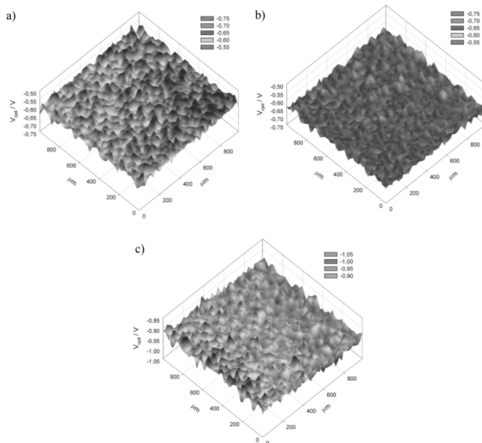
Fig. 4. Contact potential difference V_{\text{CPD}} distribution measured on Zn coating (a), as-deposited Zn-Ni coating (b) and after NSS test Zn-Ni coating (c).
