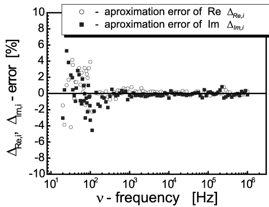
Fig. 6. The residuals plot: relative differences, \Delta_{\text{Re},i} and \Delta_{\text{Im},i} , between the impedance data and its Kramers Kronig-compliant fit plotted versus \log(\text{frequency}) .
