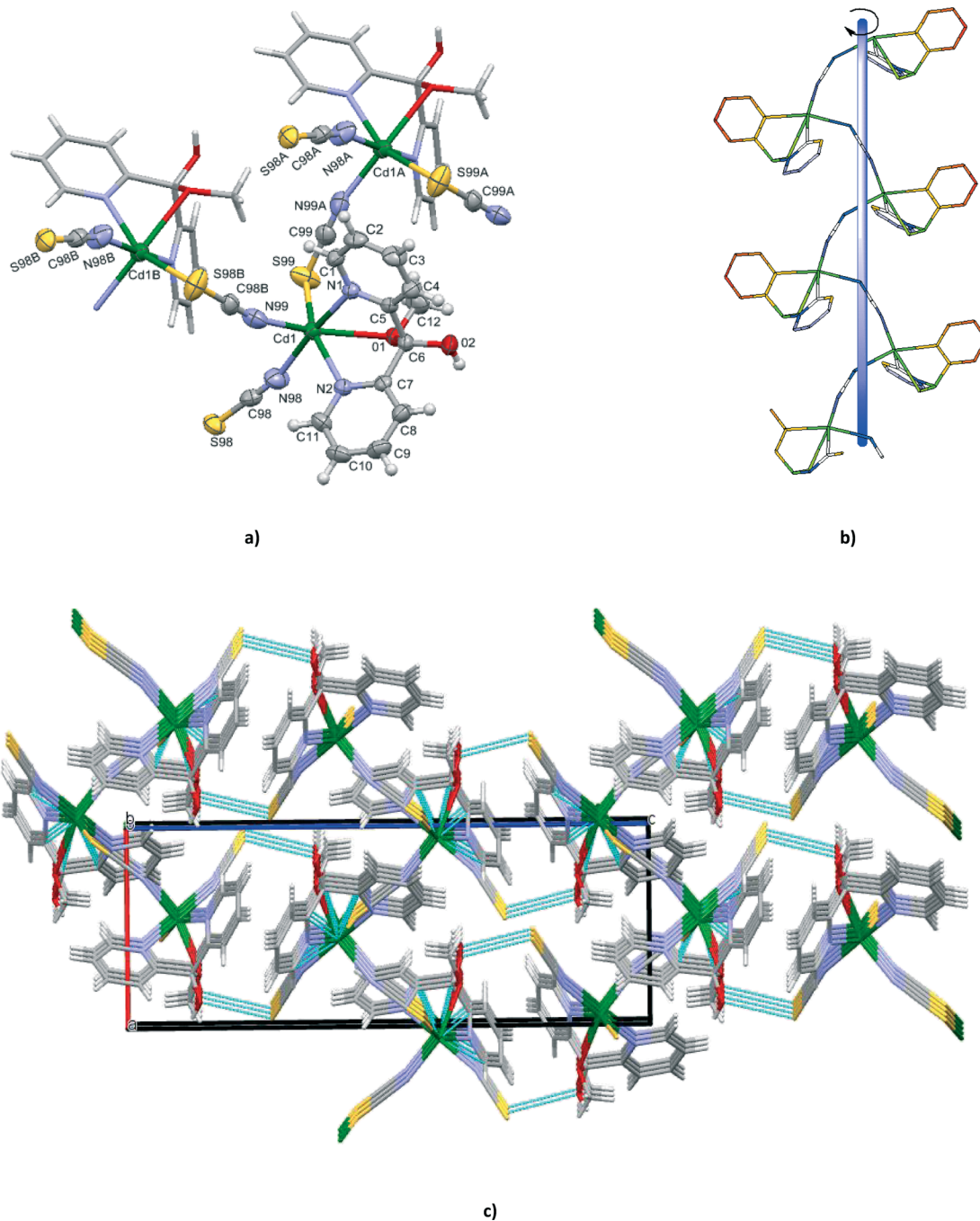
Fig. 1 (a) Perspective view of the fragment of [\text{Cd}(\text{SCN})_2((\text{py})_2\text{C}(\text{OCH}_3)(\text{OH}))]_n ( 1 ) showing the atom numbering. Displacement ellipsoids are drawn at 50% probability. Symmetry codes: (A) = x + 1/2, -y + 1/2, -z + 1 ; (B) = x - 1/2, -y + 1/2, -z + 1 ; (b) perspective view of M helix; (c) view of the three dimensional supramolecular network formed via a weak interaction \text{O}(2) \cdots \text{S}(99)^l [(i): 2 - x, 0.5 + y, 1.5 - z ] interactions shown by dotted lines.
