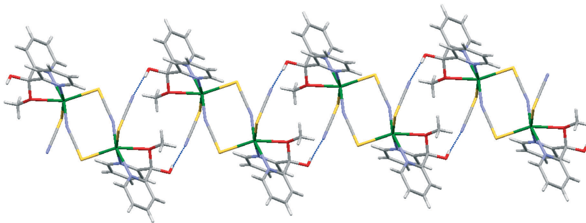
Fig. 2 (a) Molecular structure of [\text{Cd}_2(\text{SCN})_4\{(\text{py})_2\text{C}(\text{OCH}_3)(\text{OH})\}_2] ( 2 ) showing the atom numbering. Displacement ellipsoids are drawn at 50% probability. Symmetry codes: (A) = -x, -y + 1, -z + 1 ; (b) view of the packing of 2 showing the hydrogen bonds \text{O}(2)\text{-H}(2\text{A})\cdots\text{N}(98)^{\text{i}} [ \text{D}\cdots\text{A} distance = 2.769(7) Å and \text{D-H}\cdots\text{A} angle = 167.0^\circ ; (i): -x, 2 - y, 1 - z ].
