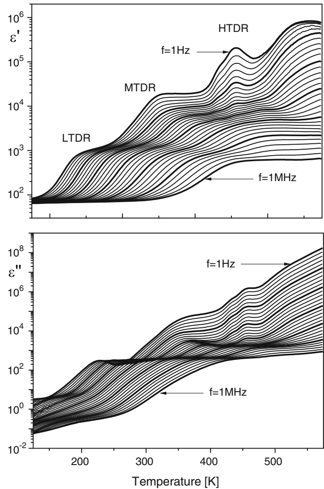
Fig. 4 Temperature dependences of real ε' and imaginary ε'' parts of dielectric permittivity of the hot-pressed BFO sample
