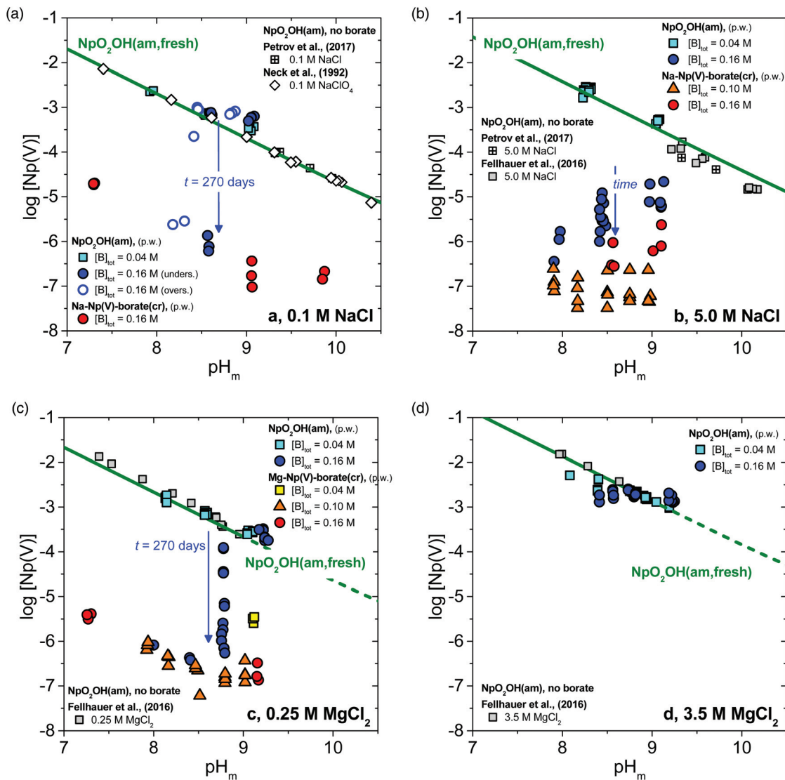
Fig. 1 Solubility of Np(v) in the presence of 0.04 M \leq [B]_{\text{tot}} \leq 0.16 M (coloured symbols) in (a) 0.1 M NaCl, (b) 5.0 M NaCl, (c) 0.25 M MgCl 2 and (d) 3.5 M MgCl 2 solutions. Solubility data obtained with NpO 2 OH(am) (blue symbols) and Na/Mg–Np(v)–borate(cr) (yellow/orange/red symbols) as Np(v) “starting material” (see text). Comparison with experimental solubility data in the absence of borate (open symbols, black) as reported by Neck et al. , (1992), 38 Petrov et al. , (2017) 39 and Fellhauer et al. , (2016). 40 Solid green line in figures (a)–(c) correspond to the solubility of NpO 2 OH(am, fresh) calculated according with thermodynamic data selected in the NEA–TDB. 16 Ionic strength in figure (d) extends well beyond the applicability of SIT, and thus the solid green line in the figure is only provided to help visualize the trend in data. In MgCl 2 solutions (figures c and d), the maximum pH m (pH max ) is limited to \approx 9 by the precipitation of Mg(OH) 2 (cr) or Mg 2 (OH) 3 Cl·4H 2 O(cr).
