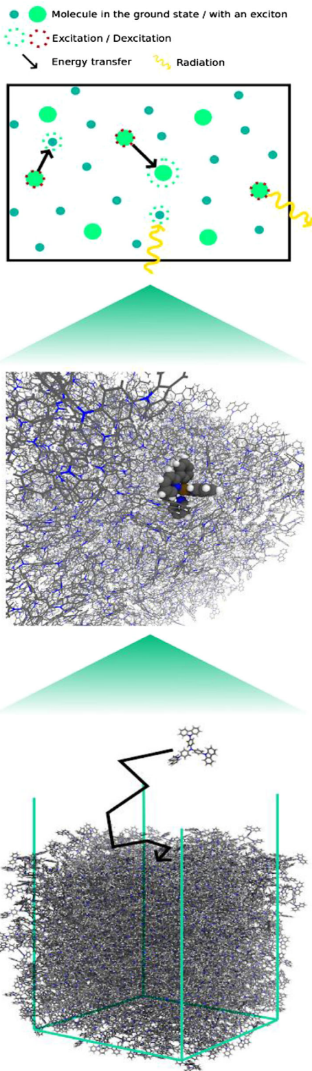
Figure 1. Multiscale simulation workflow from top down. Exciton dynamics are simulated in KMC. Excitons can be created, moved, decayed radiatively, and can undergo bimolecular quenching. Rates for these processes are computed from first principles on atomistic molecular morphologies. Morphologies are generated emulating physical vapor deposition.
