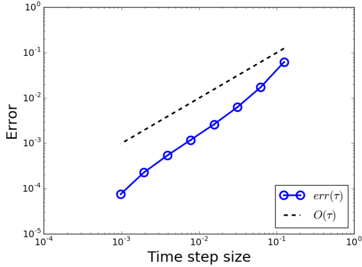
Fig. 3: Convergence plot for m .
