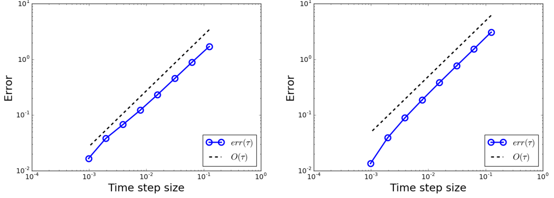
Fig. 2: Convergence plot for \varphi (left) and \psi (right).
