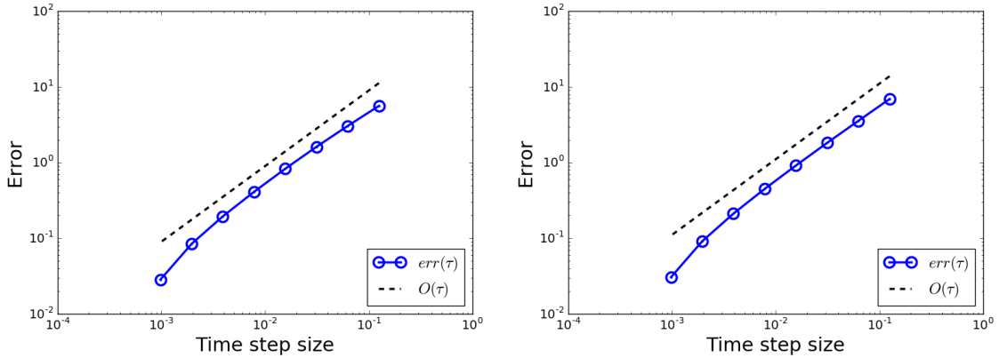
Fig. 1: Convergence plot for E (left) and H (right).
