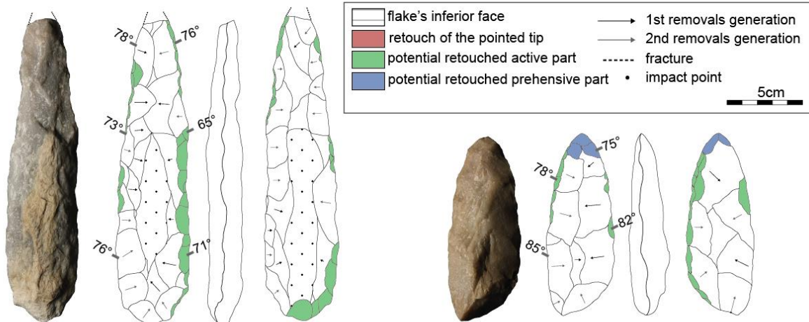
NZA21 - Partially bifacially shaped tool on slab. The knapper used the natural blank to produce a long and thin shaped tool. The distal part is broken but the overall morphology suggest a possible pointed tip.
