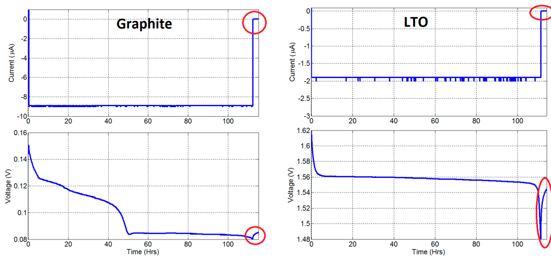
Figure A2. Terminal voltage curves of discharges at a very small current rate.
