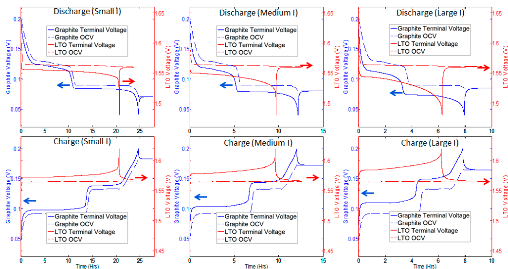
Figure 4. Terminal voltage comparison of simulated graphite and LTO half-cells cycled with constant current at 0.045 C, 0.089 C and 0.13 C.
