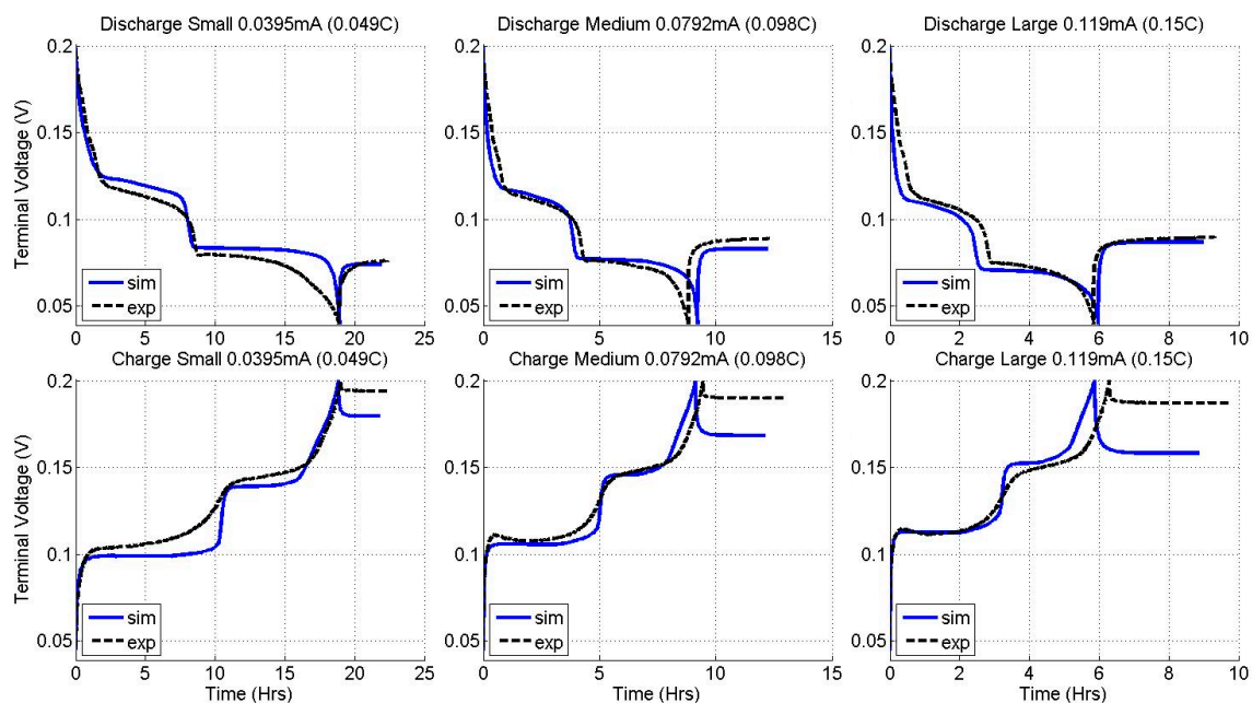
Figure 2. Experimental validation of the terminal voltage of a graphite half-cell at 0.05 C, 0.1 C and 0.15 C cycles.
