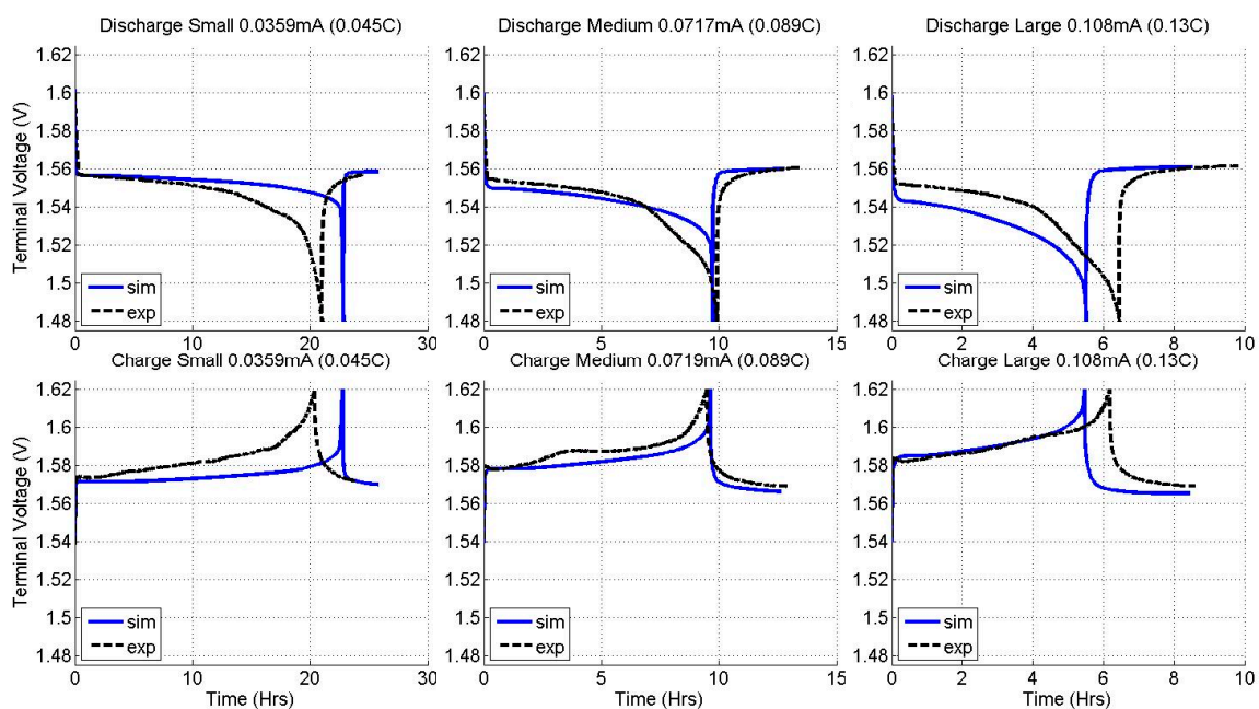
Figure A3. Experimental validation of terminal voltage of LTO half-cell without considering the current dependency of D_s .
