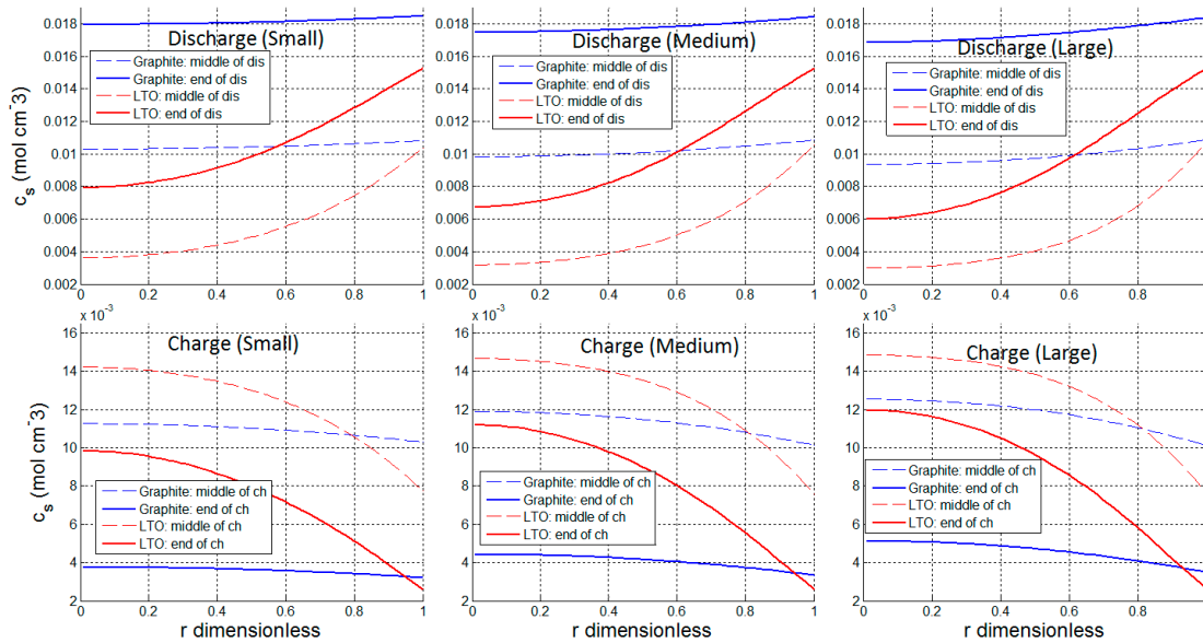
Figure 6. Ion concentrations in solid particles of graphite and LTO half-cells during 0.045 C, 0.089 C, and 0.13 C cycles.
