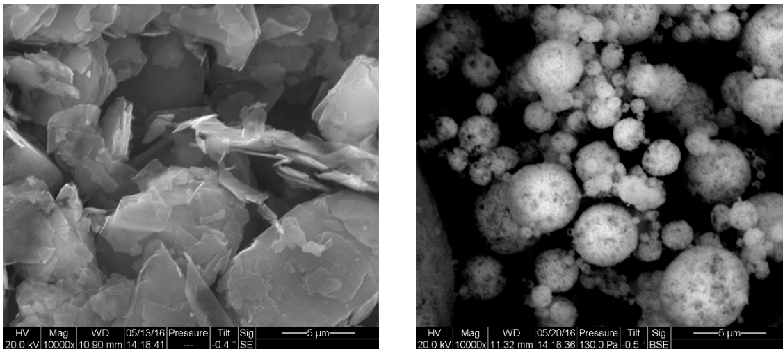
Figure A1. SEM images of: graphite particles (left); and LTO particles (right).
