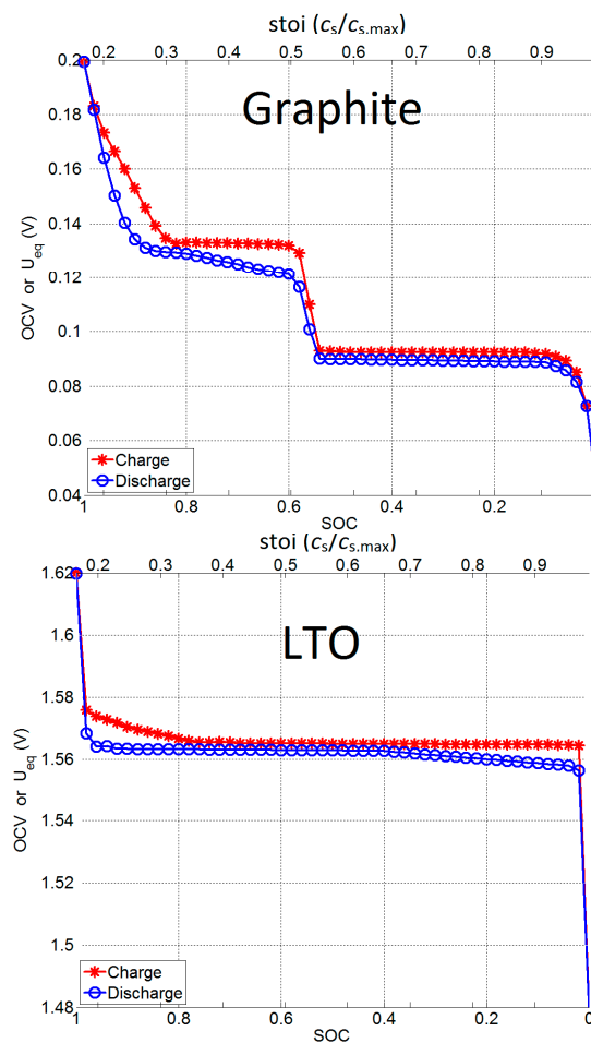
Figure 1. OCV or U_{eq} measurement vs. state of charge (SOC) for graphite and \text{Li}_4\text{Ti}_5\text{O}_{12} anode.
