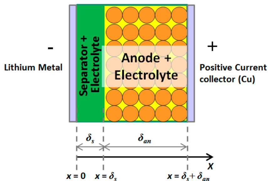
Figure 8. Geometry setup for a half-cell model with a graphite or LTO anode (single particle schematics).
