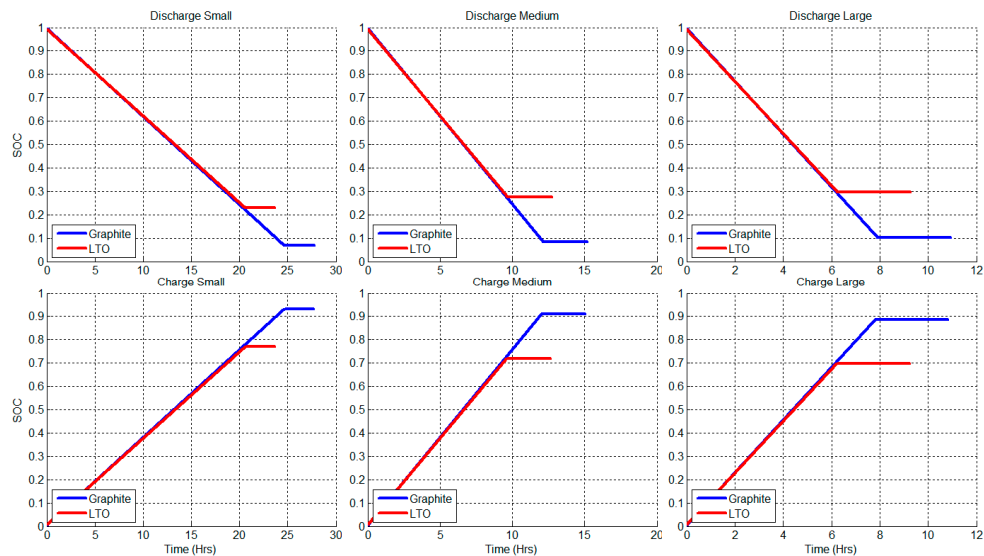
Figure 5. State of charge (SOC) comparison of graphite and LTO half-cell simulations of 0.045 C, 0.089 C, and 0.13 C cycles.
