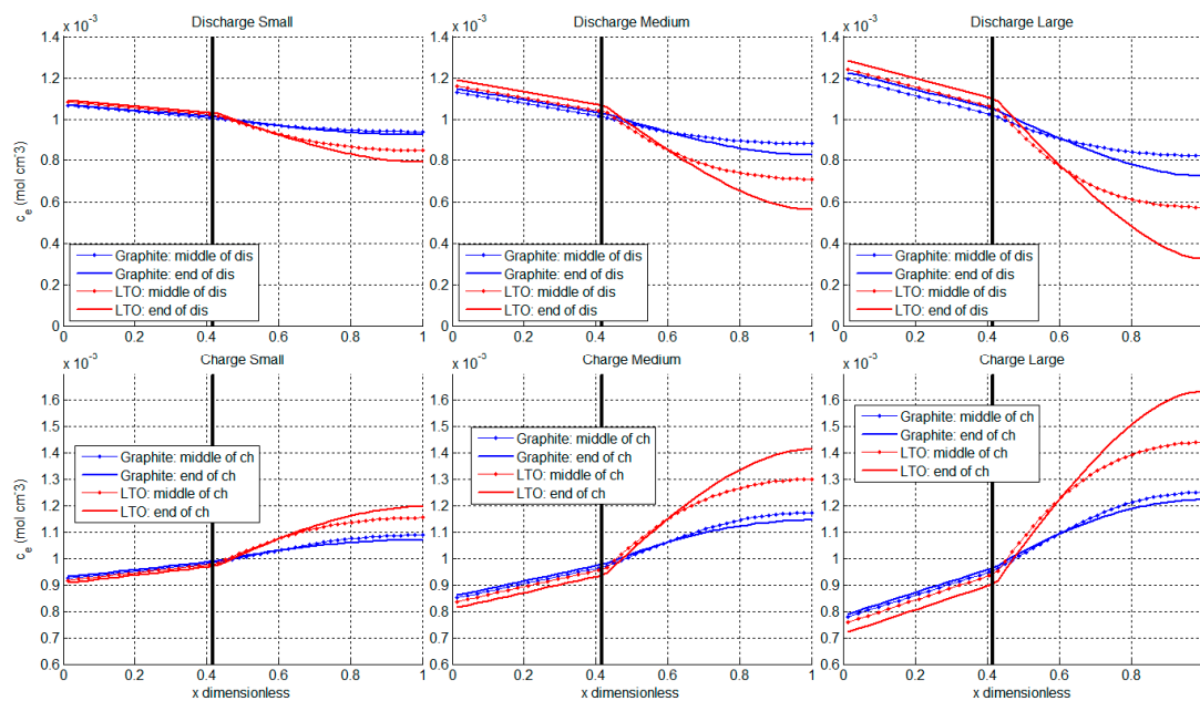
Figure 7. Ion concentrations in the electrolyte of graphite and LTO half-cells while cycling at 0.045 C, 0.089 C, and 0.13 C.
