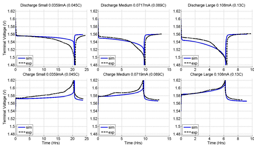
Figure 3. Experimental validation of terminal voltage of an LTO half-cell at 0.05 C, 0.1 C and 0.15 C cycles.
