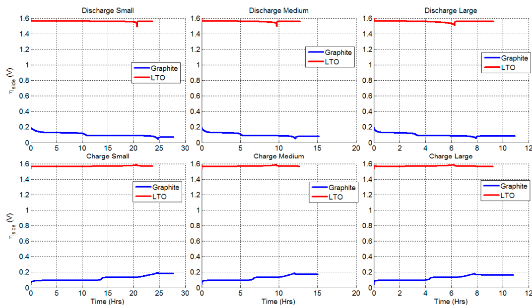
Figure 9. Activation overpotential of side reactions in graphite and LTO half-cells cycled at 0.045 C, 0.089 C, and 0.13 C.
