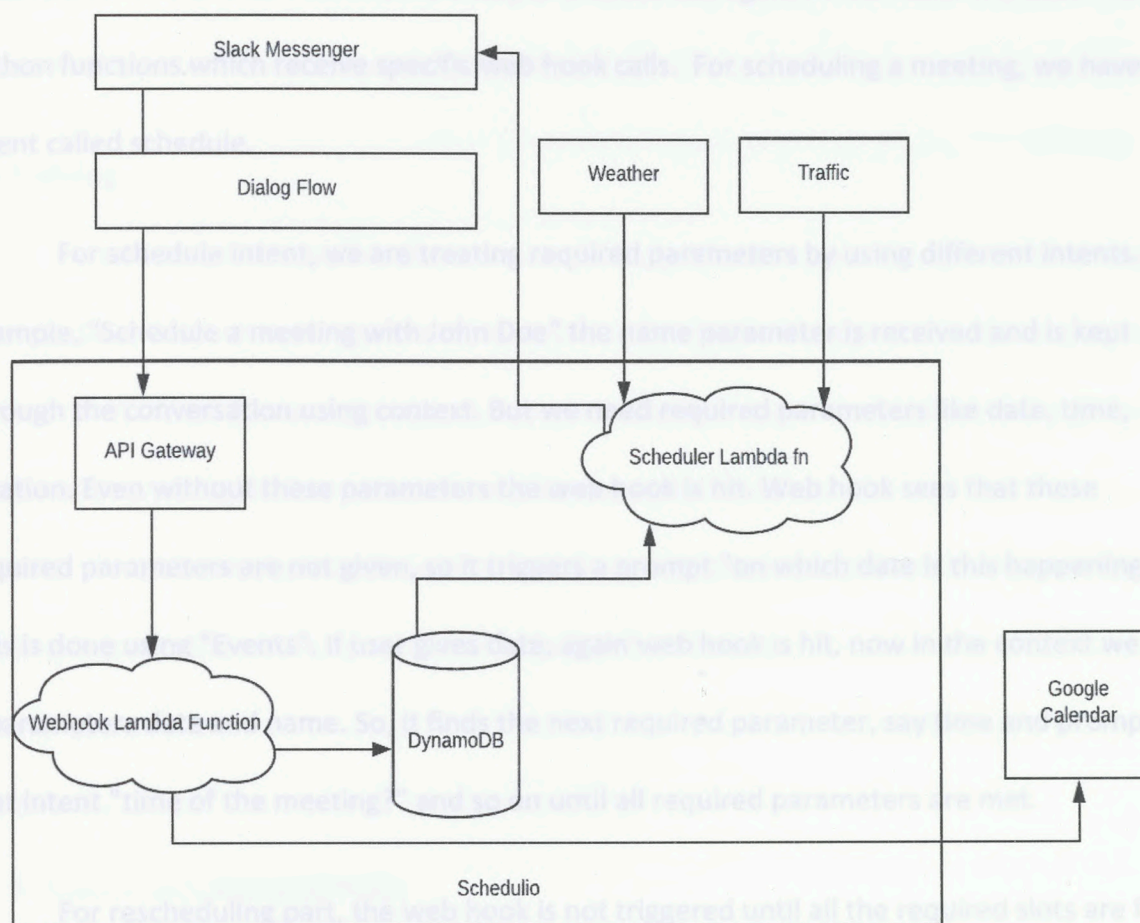
Fig. 3 Schedulio Architecture
