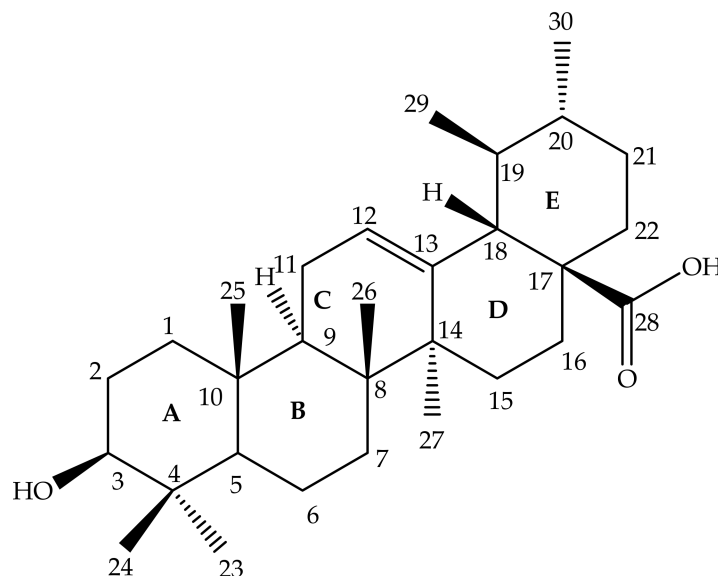
Figure 1. Ursolic acid chemical structure.
