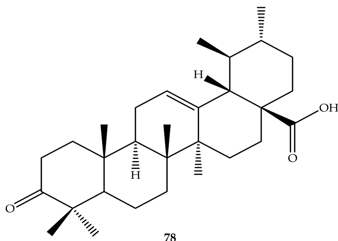
Figure 9. Some reported UA analogues.
