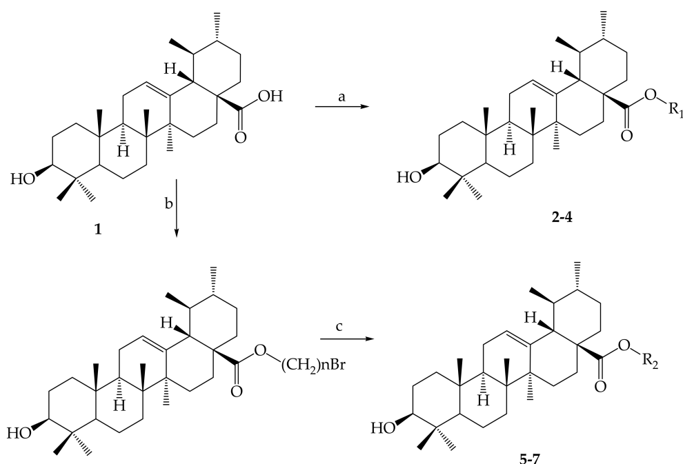
Figure 2. Preparation of UA ester derivatives. Reagents and conditions: (a) \text{CH}_3(\text{CH}_2)_n\text{Br} , potassium carbonate ( \text{K}_2\text{CO}_3 ), dimethylformamide ( (\text{CH}_3)_2\text{NCH} ); (b) \text{Br}(\text{CH}_2)_n\text{Br} , \text{K}_2\text{CO}_3 , (\text{CH}_3)_2\text{NCH} ; (c) Acetonitrile \text{CH}_3\text{CN} /silver nitrate ( \text{AgNO}_3 ), \text{COO}(\text{CH}_2)_n\text{Br} . 2: \text{R}_1 = \text{CH}_2\text{CH}_3 ; 3: \text{R}_1 = (\text{CH}_2)_2\text{CH}_3 ; 4: \text{R}_1 = (\text{CH}_2)_3\text{CH}_3 ; 5: \text{R}_2 = (\text{CH}_2)_2\text{ONO}_2 ; 6: \text{R}_2 = (\text{CH}_2)_3\text{ONO}_2 ; 7: \text{R}_2 = (\text{CH}_2)_4\text{ONO}_2 .
