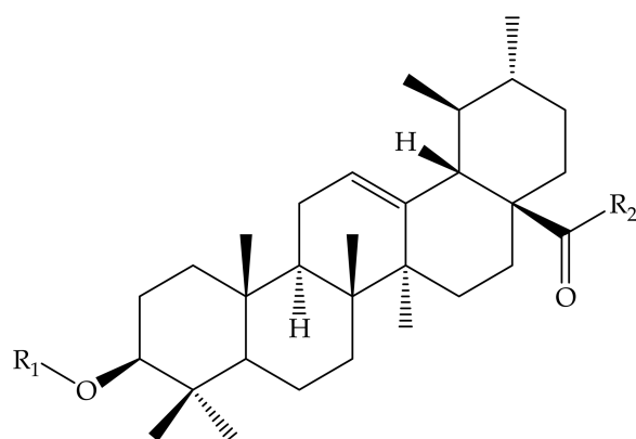
Figure 7. Synthesized UA derivatives. 42–46; 42: R 1 = COCH 3 ; R 2 = OH; 43: R 1 = COCH 2 CH 3 ; R 2 = OH; 44: R 1 = COCH 2 CH 2 CH 3 ; R 2 = OH; 5: R 1 = H; R 2 = OCH 3 ; 46: R 1 = H; R 2 = NHCH 2 CH 2 CH 3 .
