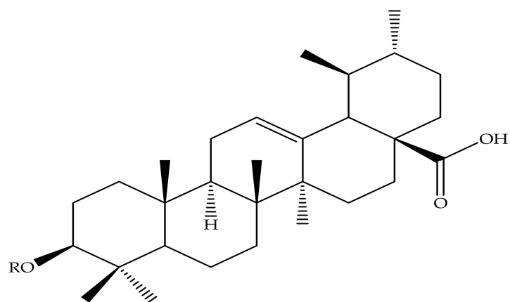
Figure 5. UA analogues. 28–29; 28: R = COH; 29: R = COCH 3 .
