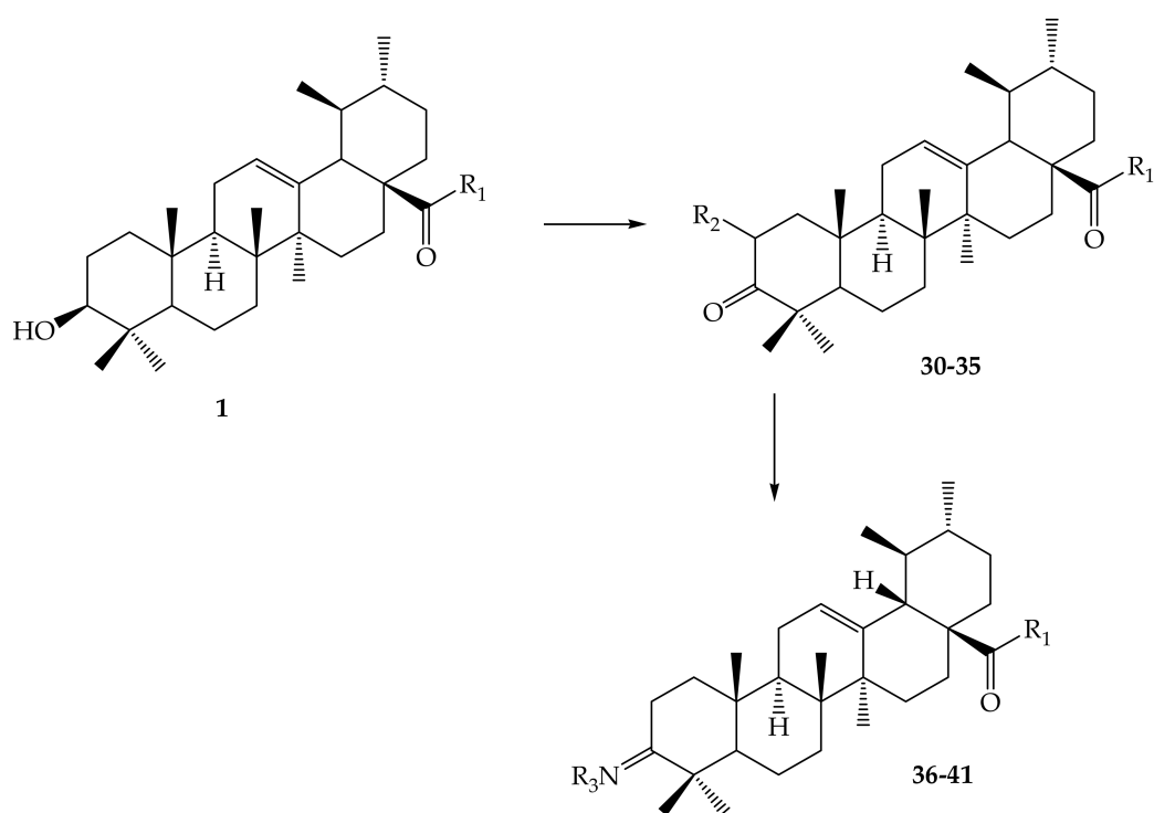
Figure 6. Derivatives synthesized from UA.
