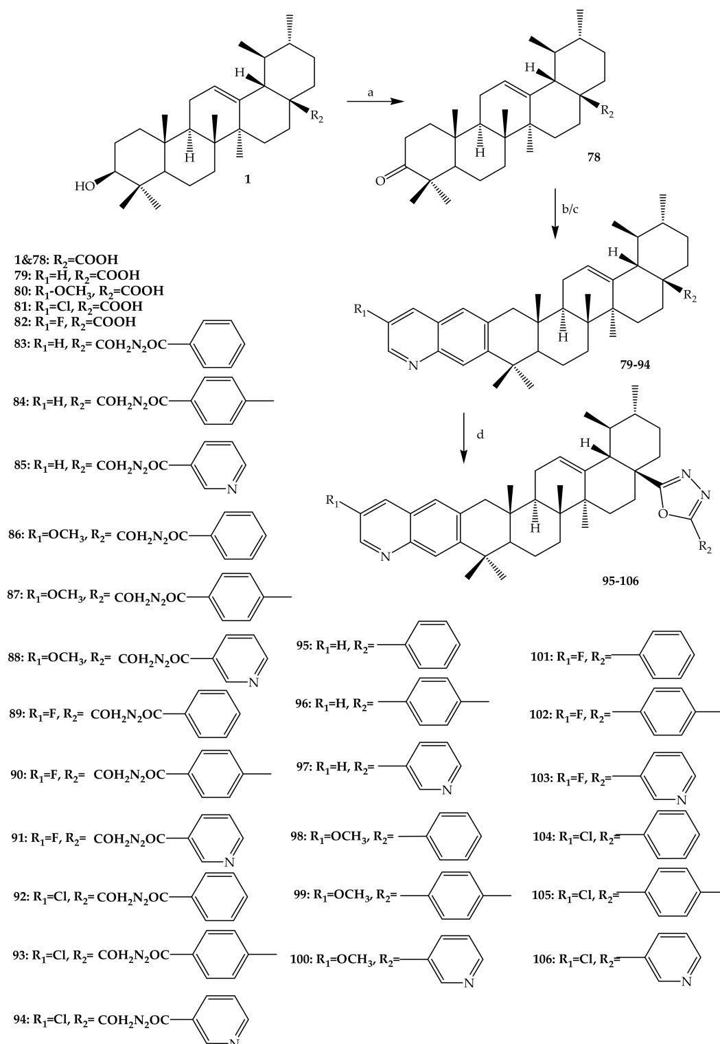
Figure 10. Summary of reaction scheme to yield UA analogues (78–106). Reagents and conditions: (a) Jones reagent, acetone at 0^\circ\text{C} for 5 h; (b) ethanol, substituted oaminobenzaldehyde, potassium hydroxide (KOH), reflux under \text{N}_2 atmospheric conditions for 24 h; (c) Thionyl chloride ( \text{SOCl}_2 ), benzene, reflux for 3 h; \text{RCONHNH}_2 , trimethylamine ( \text{Et}_3\text{N} ), dichloromethane ( \text{CH}_2\text{Cl}_2 )/ether at room temperature for 8–12 h; (d) p-Toluenesulfonic acid (TsOH), toluene, reflux for 6 h.
