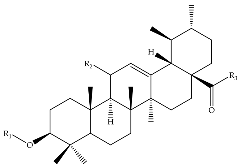
Figure 4. Some of UA derivatives. 1, 25–27; 1: R 1 = H; R 2 = H; R 3 = OH; 25: R 1 = OCCH 3 ; R 2 = H; R 3 = OH; 26: R 1 = OCCH 3 ; R 2 = O; R 3 = NHC 6 H 5 ; 27: R 1 = OCH 2 CH 2 CH 3 ; R 2 = H; R 3 = NHCH 2 CO 2 CH 3 .
