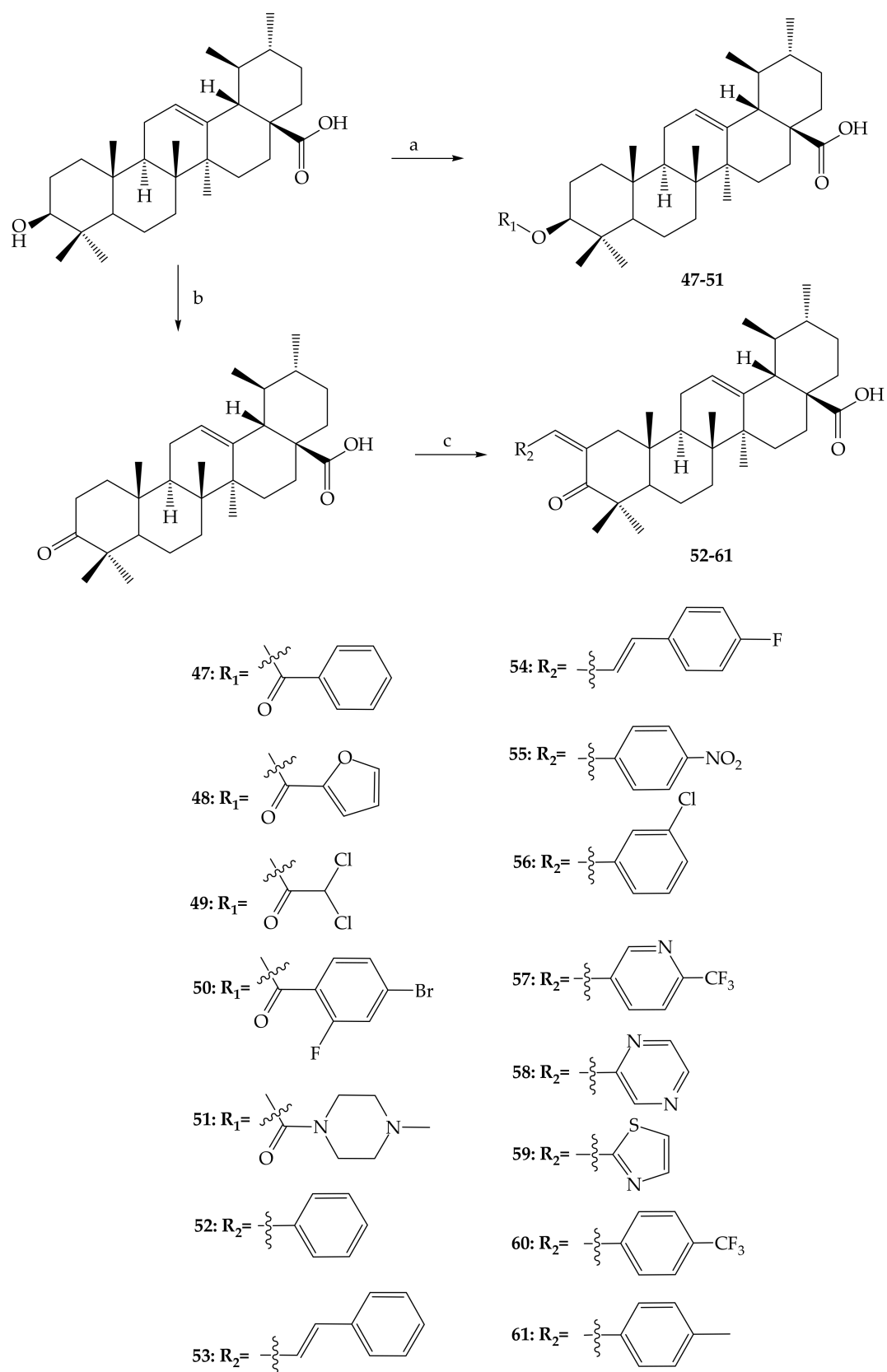
Figure 8. Synthesis of UA derivatives; reagents and conditions: (a) acid chloride or anhydride, DMAP, pyridine, reflux; (b) chromium (III) oxide (CrO 3 ), sulphuric acid (H 2 SO 4 ), acetone, 0 °C, 1 h; (c) R1-CHO, potassium hydroxide (KOH), ethanol, room temperature.
