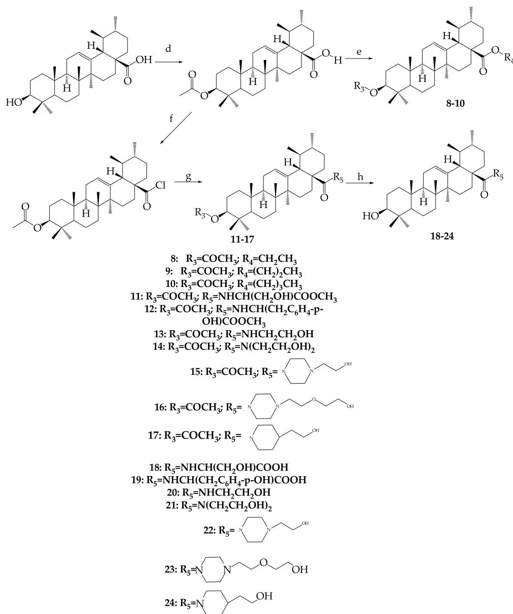
Figure 3. Modification of UA yielded amides and ester derivatives. Reagents and conditions: (d) anhydride/Pyridine/ N,N -dimethyl-4-aminopyridine (DMAP); (e) CH_3(CH_2)_nBr , K_2CO_3 , (CH_3)_2NCH ; (f) rhodium carbonyl chloride ( (CO)_2Cl ), dichloromethane ( CH_2Cl_2 ); (g) CH_2Cl_2 , triethylamine ( Et_3N ), HR; (h) NaOH, methanol ( CH_3OH )/tetrahydrofuran (THF). All the reactions were carried out at room temperature.
