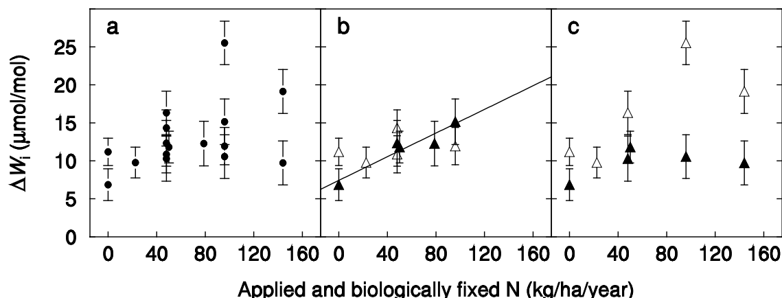
Figure 1. Relationship between the absolute change in W_i from 1915 to 2009 ( \Delta W_i , \mu\text{mol/mol} ) and the amount of applied plus biologically fixed N ( \text{kg/ha/year} ), presented for (a) all plots, (b) \text{NO}_3\text{-N} and (c) \text{NH}_4\text{-N} plots and their limed ( \blacktriangle ) and unlimed ( \triangle ) subplots. The same data from the controls and the PK-only plots are used in all three graphs. The black line is the linear regression for the limed \text{NO}_3\text{-N} plots ( y = 7.43 + 0.08x , P < 0.05 , R^2 = 0.9 ). Error bars represent the standard error.
