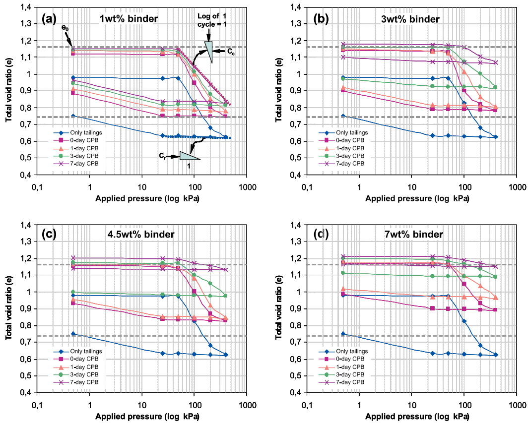
Fig. 2. Consolidation curves of CPB samples
