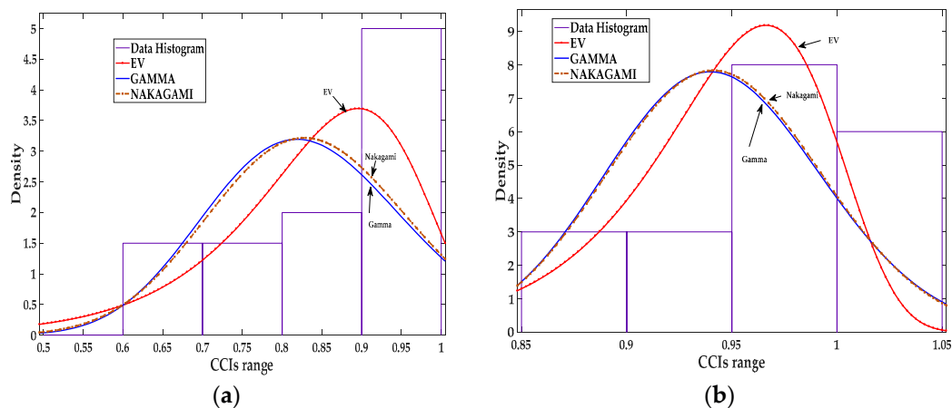
Figure 3. Data fitting for the CCIs of sensor 5: (a) Data fitting for three distributions, EV, Gamma, and Nakagami in scenario NS1P3 for NUT 13; (b) Data fitting for three distributions, EV, Gamma, and Nakagami in scenario NS15P7 for NUT 19.
