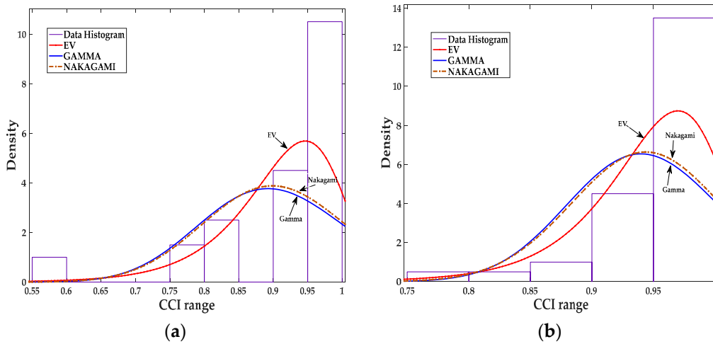
Figure 4. Data fitting for the CCIs of sensor 5: (a) Data fitting for three distributions, EV, Gamma, and Nakagami in scenario NS5P7 for NUT 13; (b) Data fitting for three distributions, EV, Gamma, and Nakagami in scenario NS5P7 for NUT 19.
