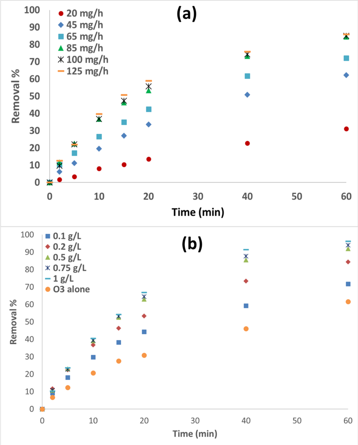
Figure 2.6 a) Effect of ozone dosage on phenol removal in the O 3 /GO/MgO process (experimental conditions: GO/MgO: 0.2 g/L, phenol concentration: 500 mg/L, Volume: 100 mL, Temperature: 20 °C, and pH: uncontrolled). b) Effect of catalyst dosage on phenol removal in the O 3 /GO/MgO
