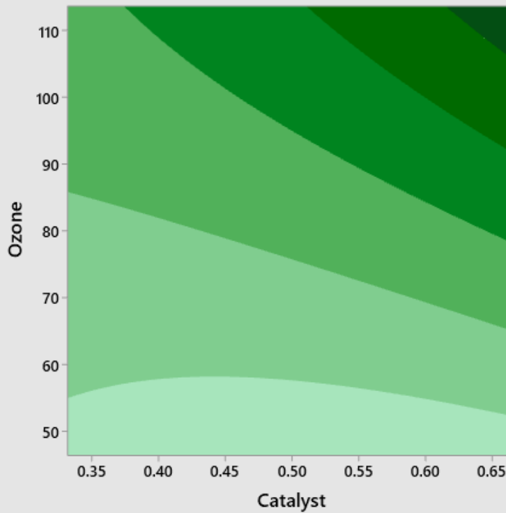
Contour Plot of Removal % vs Ozone, Catalyst
