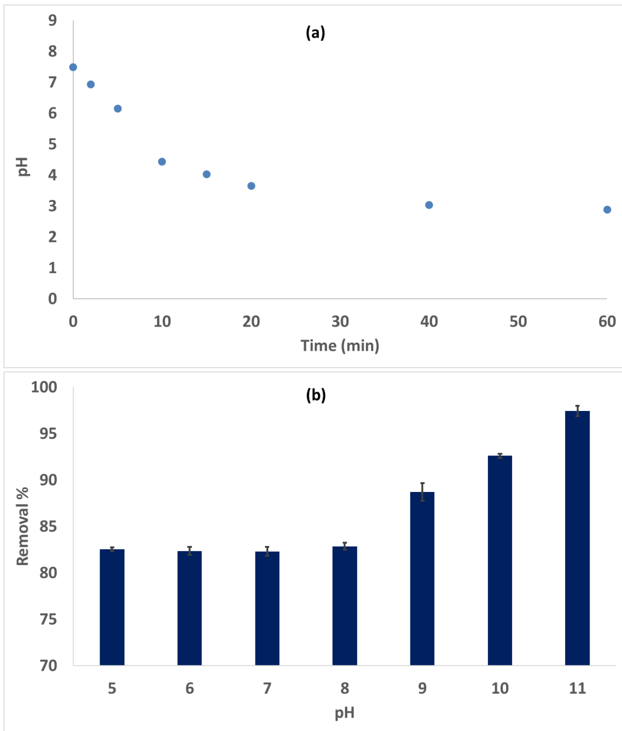
Figure 2.8 (a) Variation of pH value for the phenol solutions during O_3/GO/MgO process. The initial pH is uncontrolled. (b) Removal of phenol in O_3/GO/MgO process at various pH values. (experimental conditions: the flowing rate of O_3 : 85 mg/h, GO/MgO dosage: 0.5 g/L, phenol concentration: 500 mg/L, Volume: 100 mL, Temperature: 20 °C)
