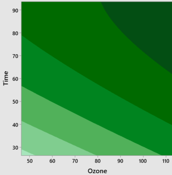
Contour Plot of Removal % vs Time, Ozone
