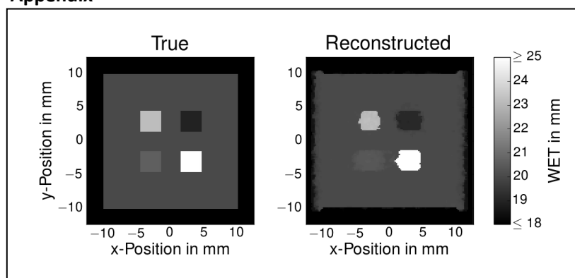
Fig.1: True/Reconstructed WET-distribution.
