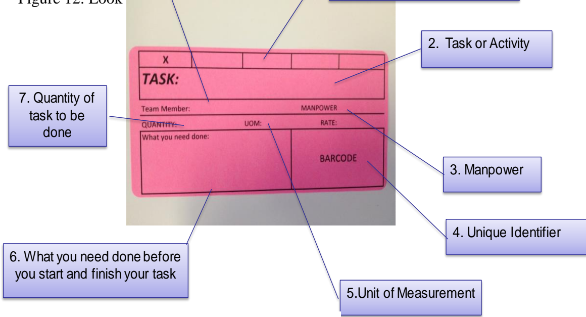
Figure 13. Pull Planning
