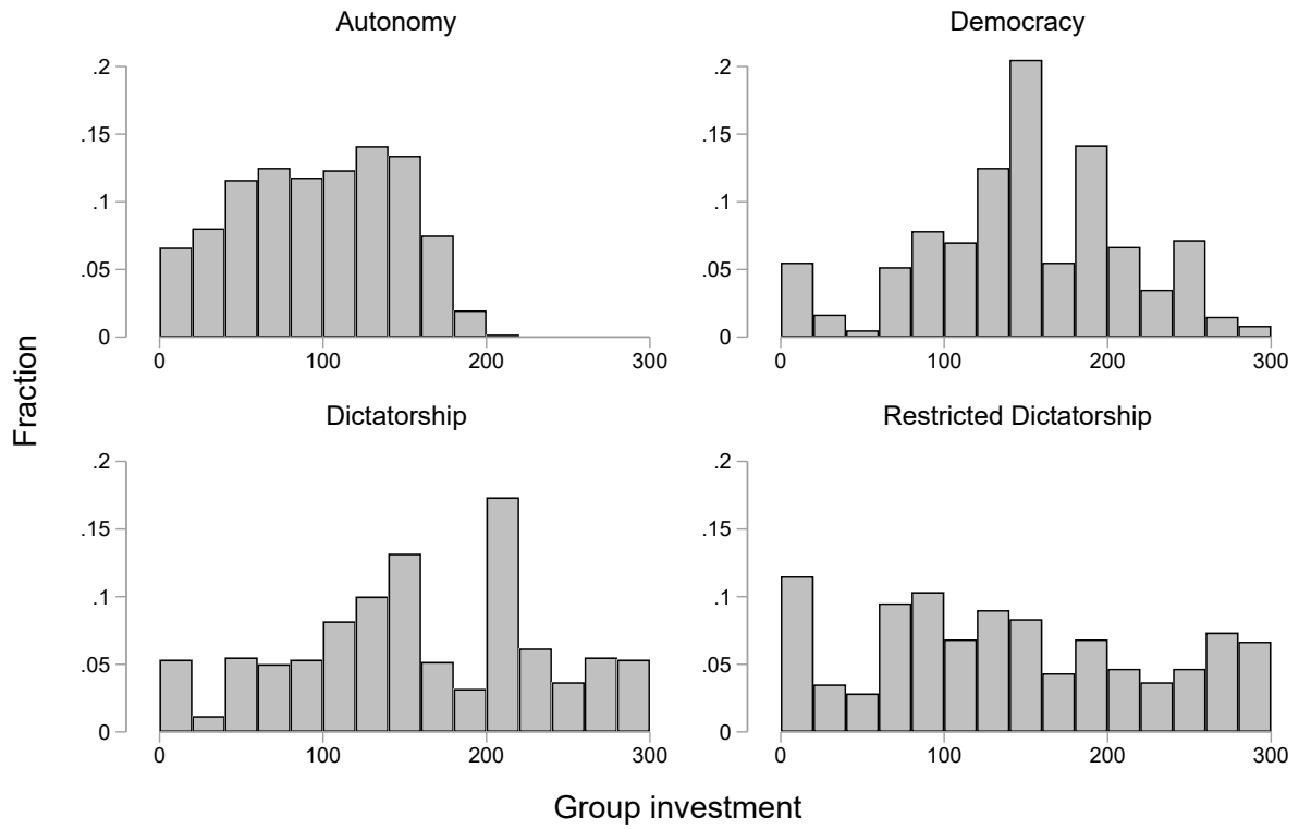
Figure A1: Distribution of total group investments in part 1 for each of the four institutions.
