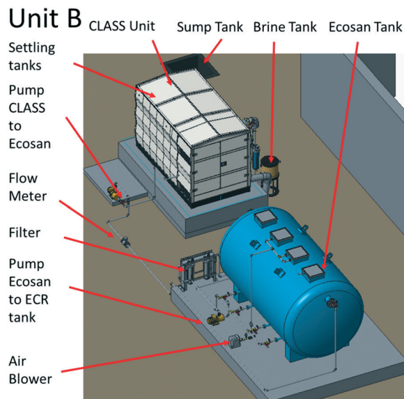
Fig. 3 Layout of the installation at site B with an EcoSan biodigester.
