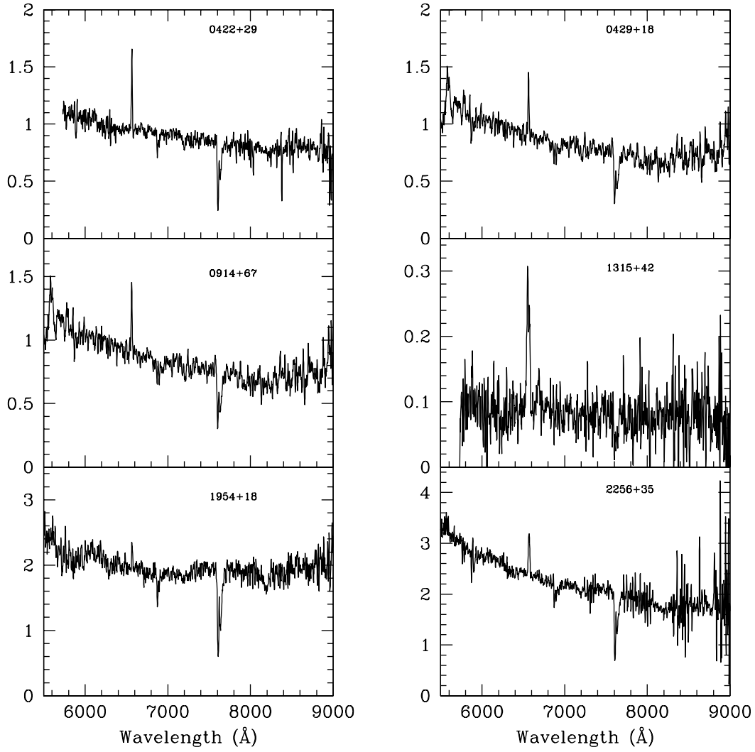
Figure 4. Red only spectra obtained at APO. The vertical axis is F_\lambda in units of 10^{-16} ergs \text{cm}^{-2} \text{s}^{-1} \text{\AA}^{-1} .
