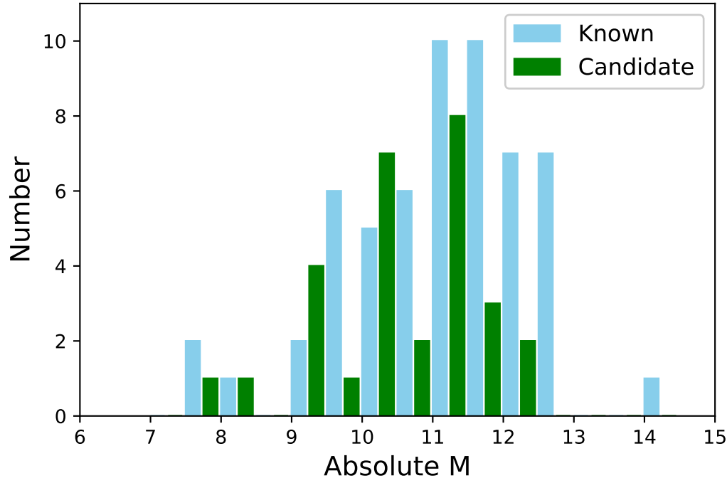
Figure 6. The number of systems in Tables 1 and 2 as a function of their absolute magnitude (in 0.5 mag bins) as determined from available Gaia parallaxes. Note that 5\sigma upper limits on the magnitudes for the fainter sources means that they are only brighter limits to the true absolute magnitude at quiescence.
