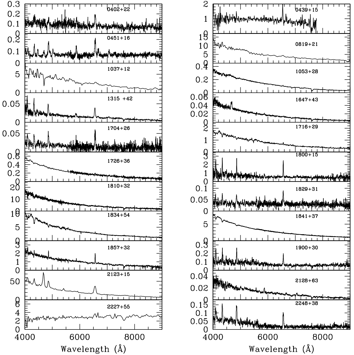
Figure 3. Blue and red spectra from Keck, Pal200in, WHT, APO, SEDM, SPRAT showing at least one Balmer or Helium emission line. The vertical axis is F_\lambda in units of 10^{-16} ergs \text{cm}^{-2} \text{s}^{-1} \text{\AA}^{-1} except for the SPRAT spectrum of ZTF0439+15 which is normalized in its reduction procedure.
