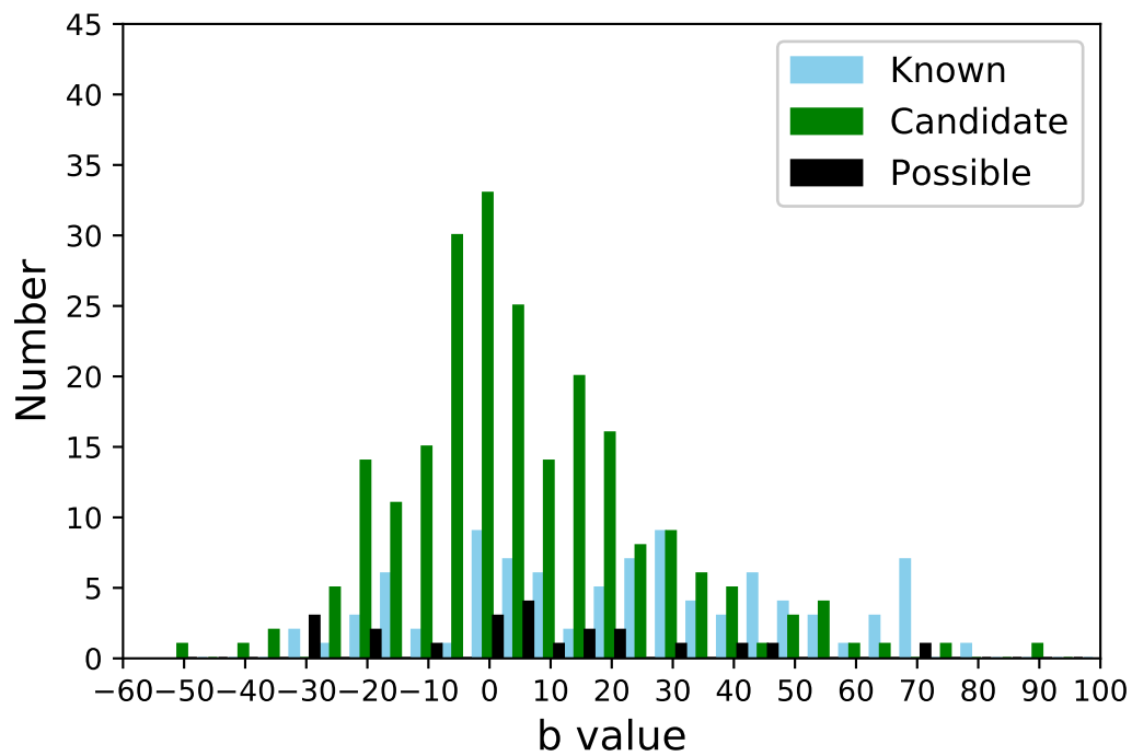
Figure 5. The number of systems in Tables 1-3 as a function of galactic latitude (in 10 deg bins).
