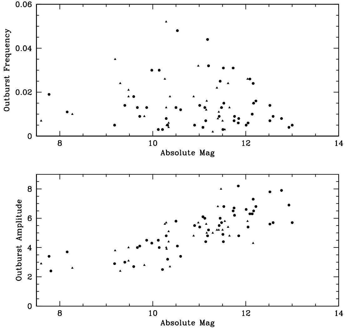
Figure 7. Plots of Absolute magnitude versus Outburst Frequency (top) and Absolute Magnitude versus Outburst Amplitude (bottom) for the objects showing dwarf nova type outbursts in Table 1 (solid dots) and Table 2 (triangles).
