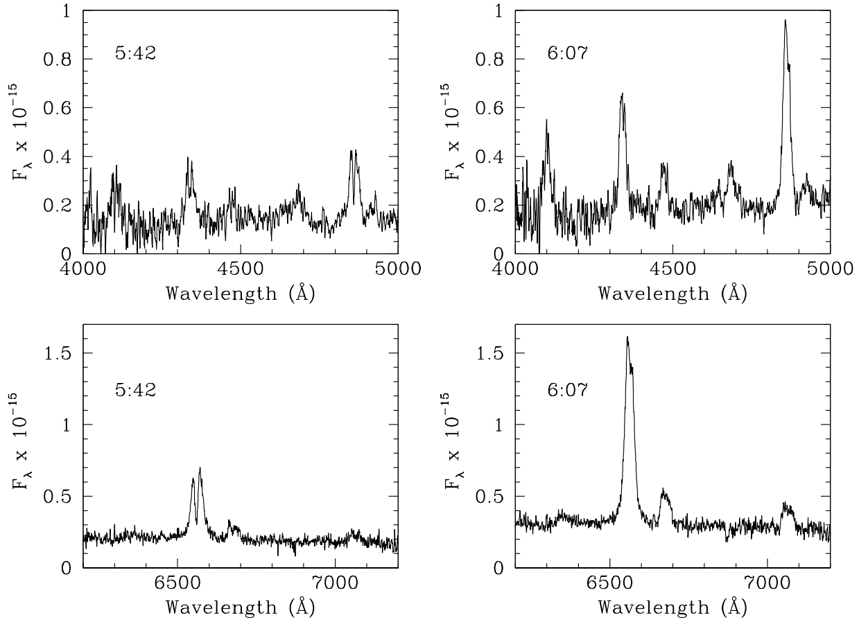
Figure 8. Two of the blue and red APO DIS spectra of 1631+69 obtained 25 min apart showing the large changes in the Balmer and He lines.
