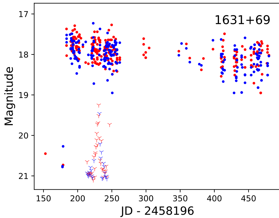
Figure 2. An example of a system showing high and low states. Symbols same as Figure 1.
