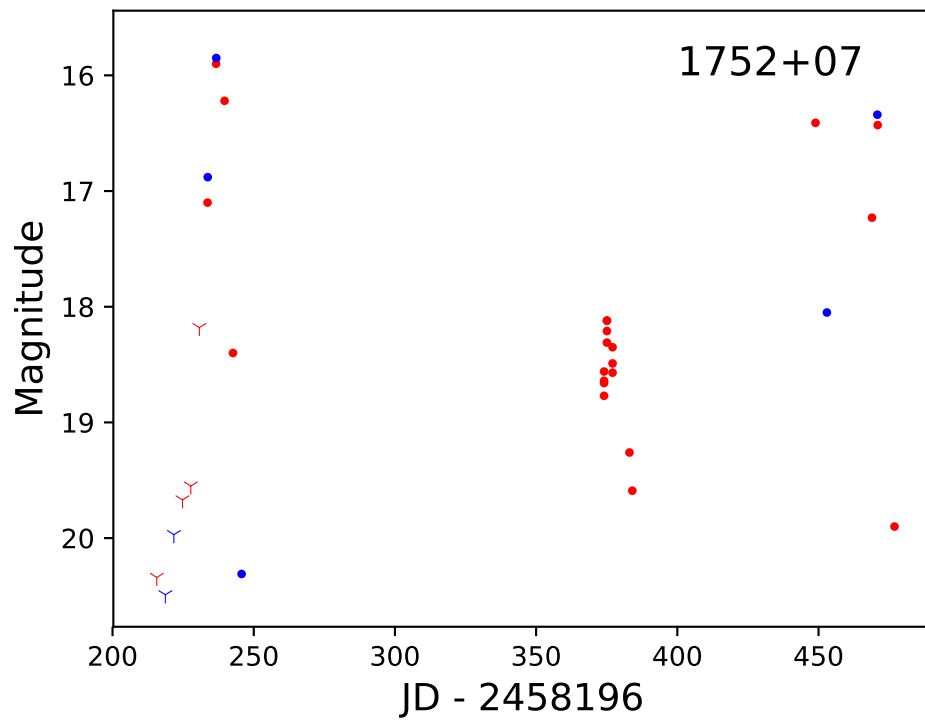
Figure 9. ZTF1752+07 (V982 Oph) light curve showing 4 dwarf nova type outbursts. Symbols same as Figure 1.
