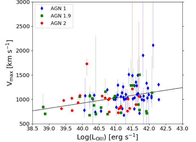
Figure 11. Outflow velocities as a function of \log L_{[\text{O III}]} for the different AGN types. We consider here the narrow component of the [O III] line.
