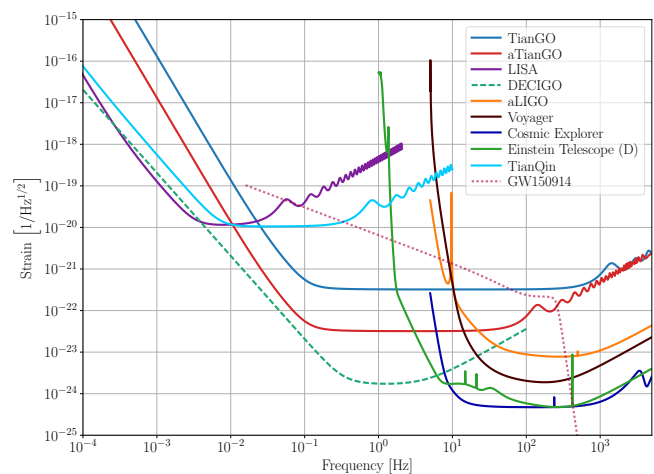
FIG. 1. Sensitivities of future ground and space gravitational wave detectors. The sensitivities are averaged over sky location and polarization. The LISA curve includes two 60^\circ interferometers and the ET curve includes three 60^\circ interferometers. The curve labeled “GW150914” is 2\sqrt{f}h , where h is the waveform of the first gravitational wave detected [18] starting five years before merger.
