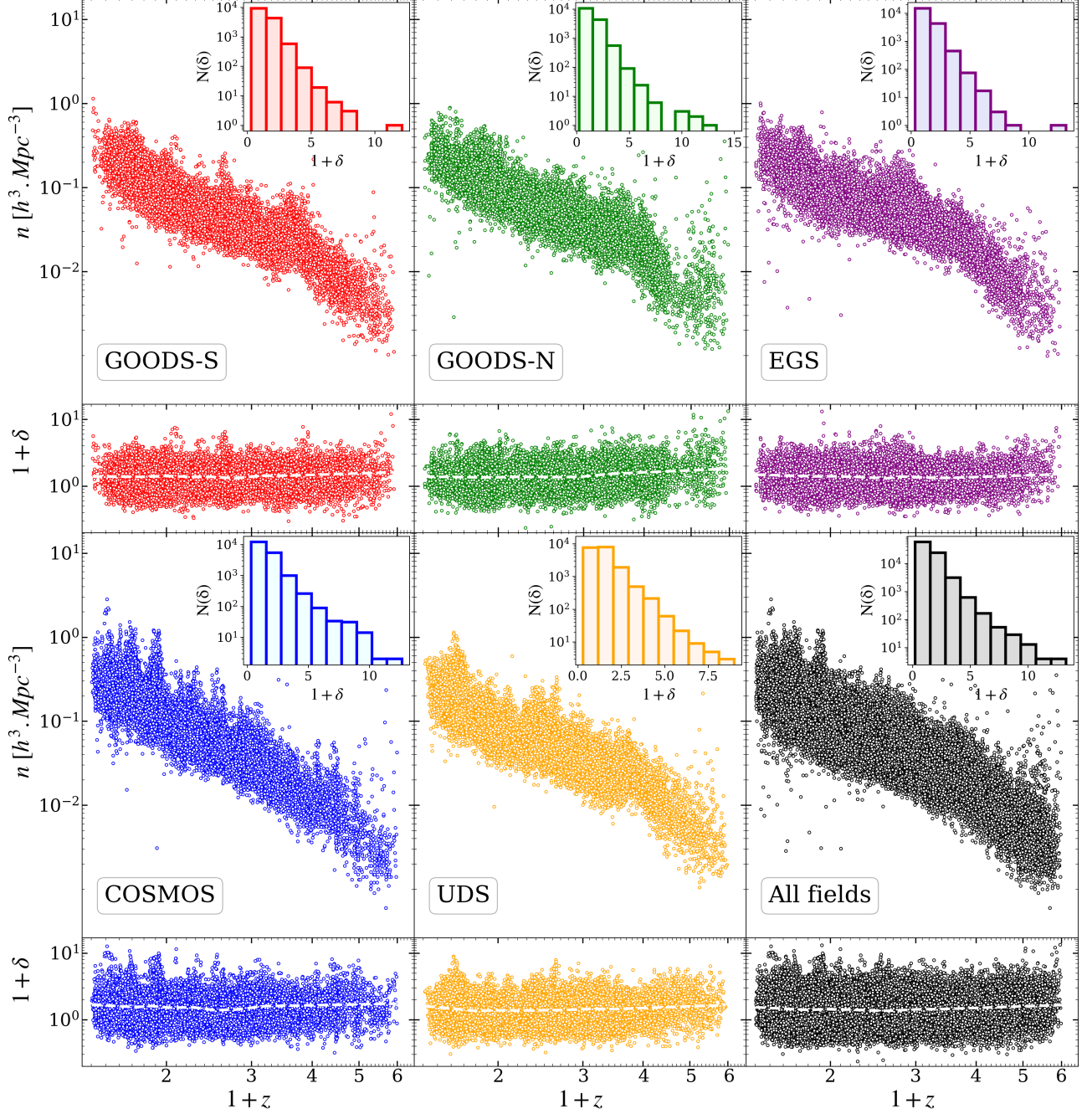
Figure B.1. The comoving number density and the density contrast as a function of redshift as well as the density contrast histogram for each field. The comoving number density decreases with redshift due to the magnitude limit of the survey, while the average density contrast (white dashed lines) is almost constant over the cosmic time. This can be explained by the weak dependence of the stellar mass function on the environment. For all the fields, we find a similar distribution of density contrast, which has a dynamic range of \sim 10 .
