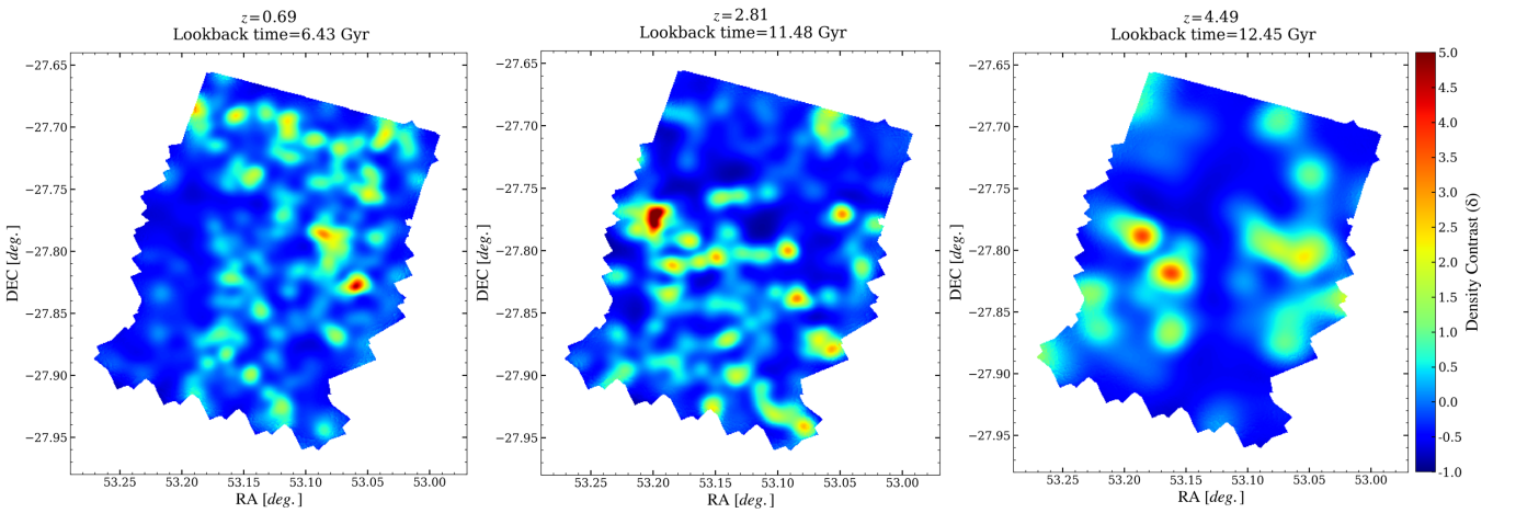
Figure A.1. Density maps, plots for the 124 redshift slices are available in an animation format in the online version.
