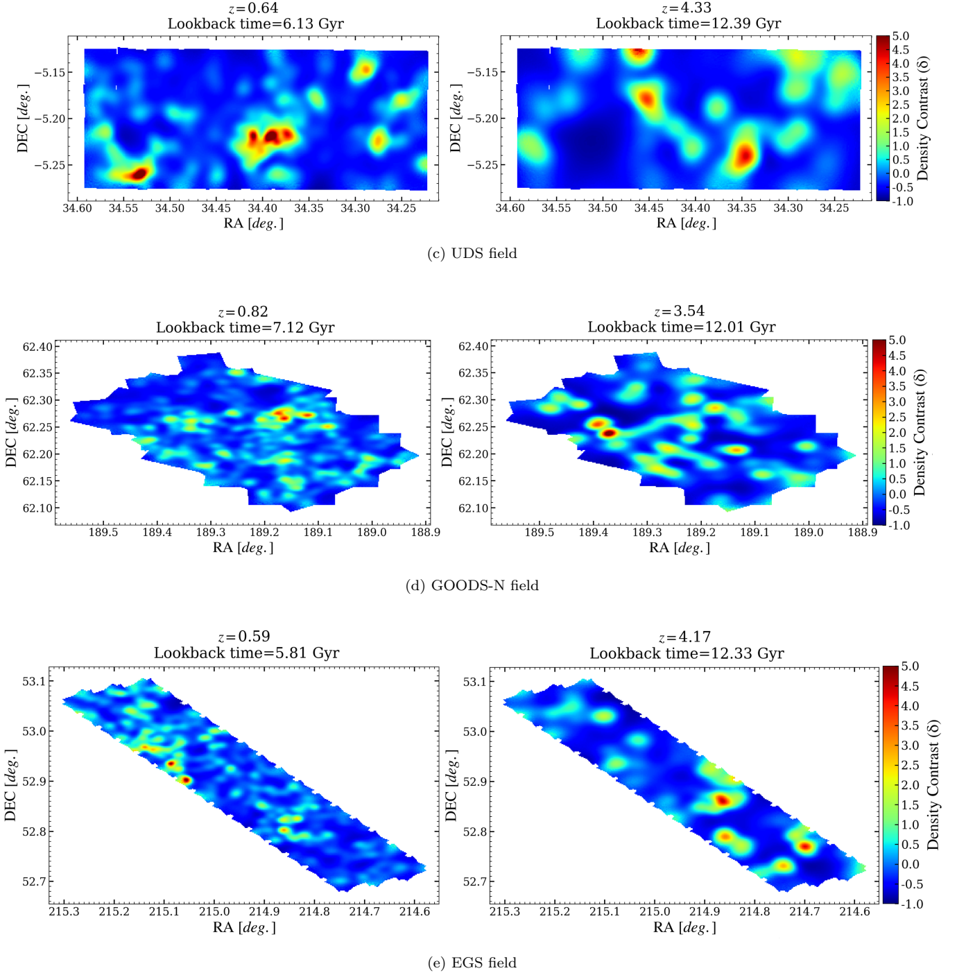
Figure A.1. Continued: Density maps, plots for the 124 redshift slices are available in an animation format in the online version.
