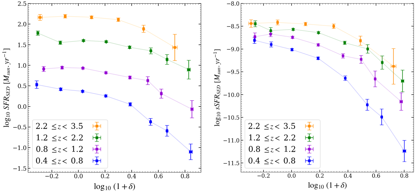
Figure 6. Environmental dependence of SFR and sSFR for a mass-complete sample of galaxies (Table 3) at four redshift bins spanning across the redshift range of z = 0.4 to z = 3.5 . The average SFR and sSFR of galaxies in density contrast bins are plotted as a function of overdensity ( 1 + \delta ). Error bars show the statistical uncertainty of the average values.
