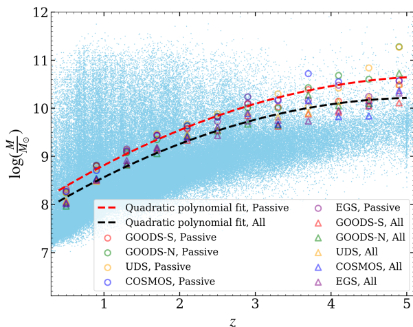
Figure 2. The stellar mass of galaxies as a function of their redshifts. Red (black) dashed line represents the 95% stellar mass completeness limit ( H_{\text{lim}} = 26 ) for the passive (all) galaxies, determined using the method of Pozzetti et al. (2010).
