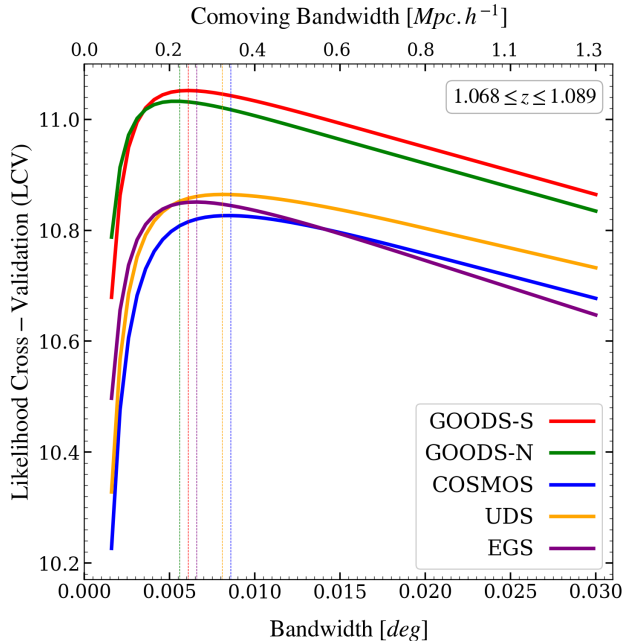
Figure 3. An example of Likelihood Cross-Validation optimization procedure at a given z -slice: 1.068 \leq z \leq 1.089 . We perform a grid search in the range of 0.0001^\circ \leq \text{Bandwidth} \leq 0.03^\circ with 50 steps to maximize the LCV and find the best bandwidth (b). Dashed vertical lines show optimized bandwidths at z \sim 1 .
