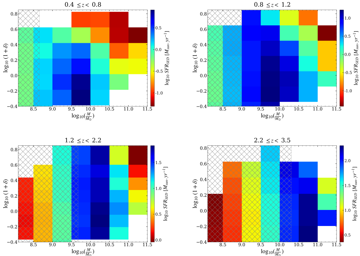
Figure 7. Average star formation rate in the bins of stellar mass and environment in four redshift intervals. The grey shaded regions show the incomplete stellar mass ranges. At all redshifts, we observe both environmental quenching and mass quenching for massive galaxies. We also find strong evidence of environmental quenching for low mass galaxies at low redshift.
