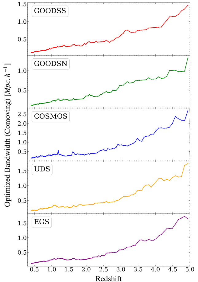
Figure 4. Optimized comoving global bandwidth (b) as a function of redshift for the five CANDELS fields. As we go to higher redshifts, we should increase the comoving size of the kernel function bandwidth to avoid the undesirable variance.
