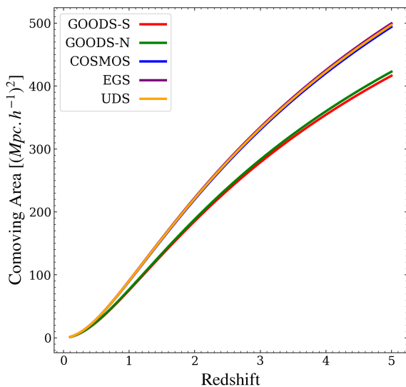
Figure 1. The comoving areal cover of the fields as a function of redshift. Each field covers \sim 25h^{-2} Mpc 2 comoving area at z \sim 0.5 up to \sim 450h^{-2} Mpc 2 at z \sim 5 .
