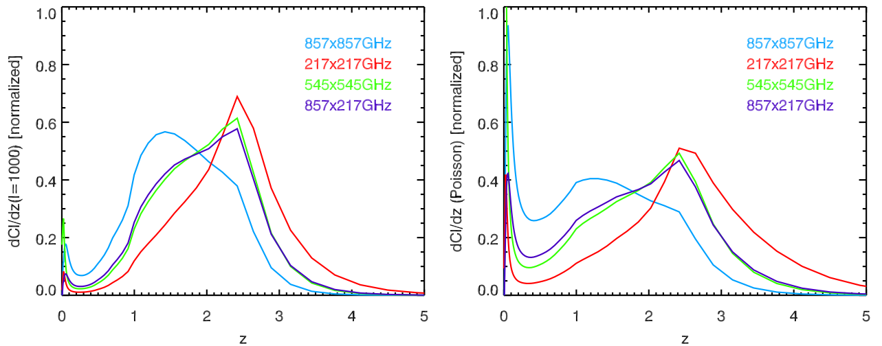
Fig. 13. Predicted redshift distribution of auto and cross power spectra at large ( \ell = 1000 , left) and small scale (Poisson level). We focus on three frequencies: 857 GHz ( 350\ \mu\text{m} ), 545 GHz ( 550\ \mu\text{m} ), and 217 GHz ( 1382\ \mu\text{m} ) to illustrate the difference between cross spectrum between two distant wavelengths and the auto-spectrum at an intermediate wavelength. The flux density cuts are the same as previously (see Sect. 6 and Fig. 7).
