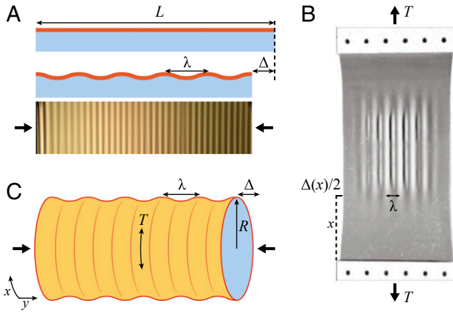
Fig. 1. Parallel wrinkles with three different sources of substrate stiffness: (A) elastic or gravitational forces, (B) tensile stresses, or (C) curvature. The examples shown are for (A) uniaxial compression of a floating sheet (e.g., from ref. 27), (B) a rectangular sheet that is clamped along two edges and stretched, and (C) the cylindrical setup discussed in Theory . In all examples, a fraction \Delta = \Delta/L of the sheet's length in the confined direction is absorbed by wrinkles. B is reprinted with permission from ref. 33.
