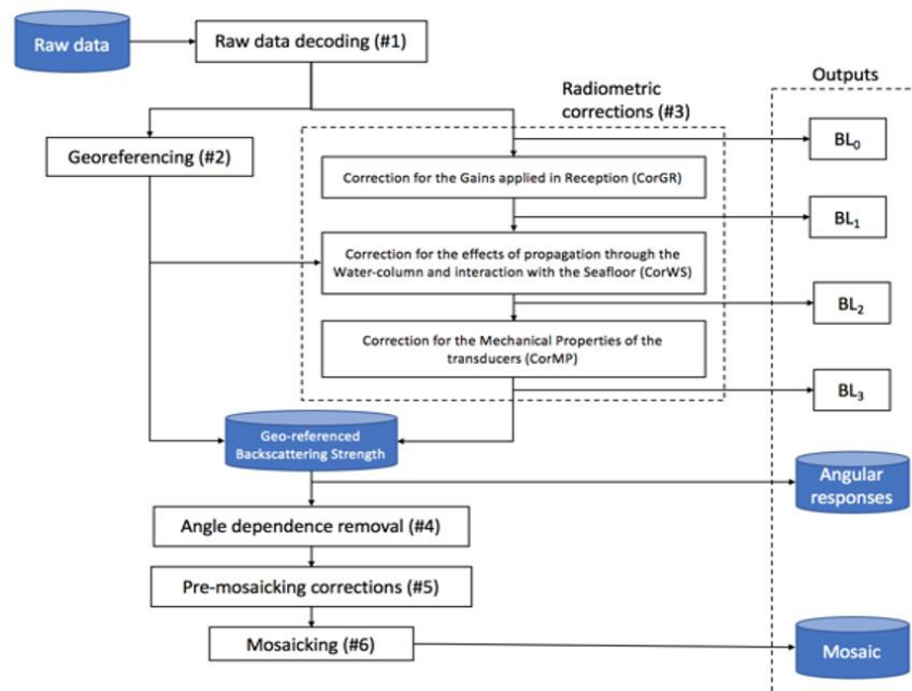
Figure 5.1: Visual workflow of the backscatter data processing pipeline (adapted from Figure 1 in [41]), resulting in the two common backscatter products: angular response curves and mosaic. Only the BL_0 and BL_3 intermediate outputs were requested from software developers during the current study.
