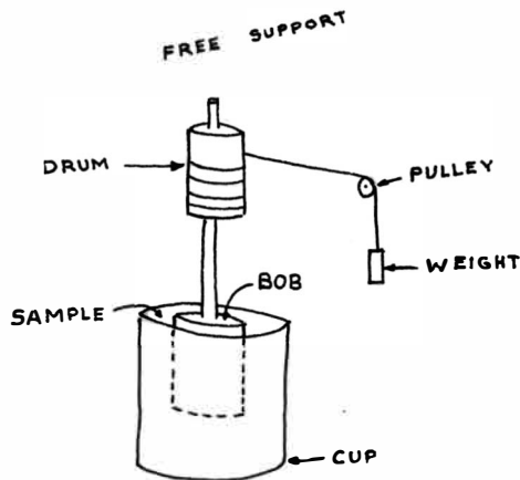
MODIFIED STORMER
