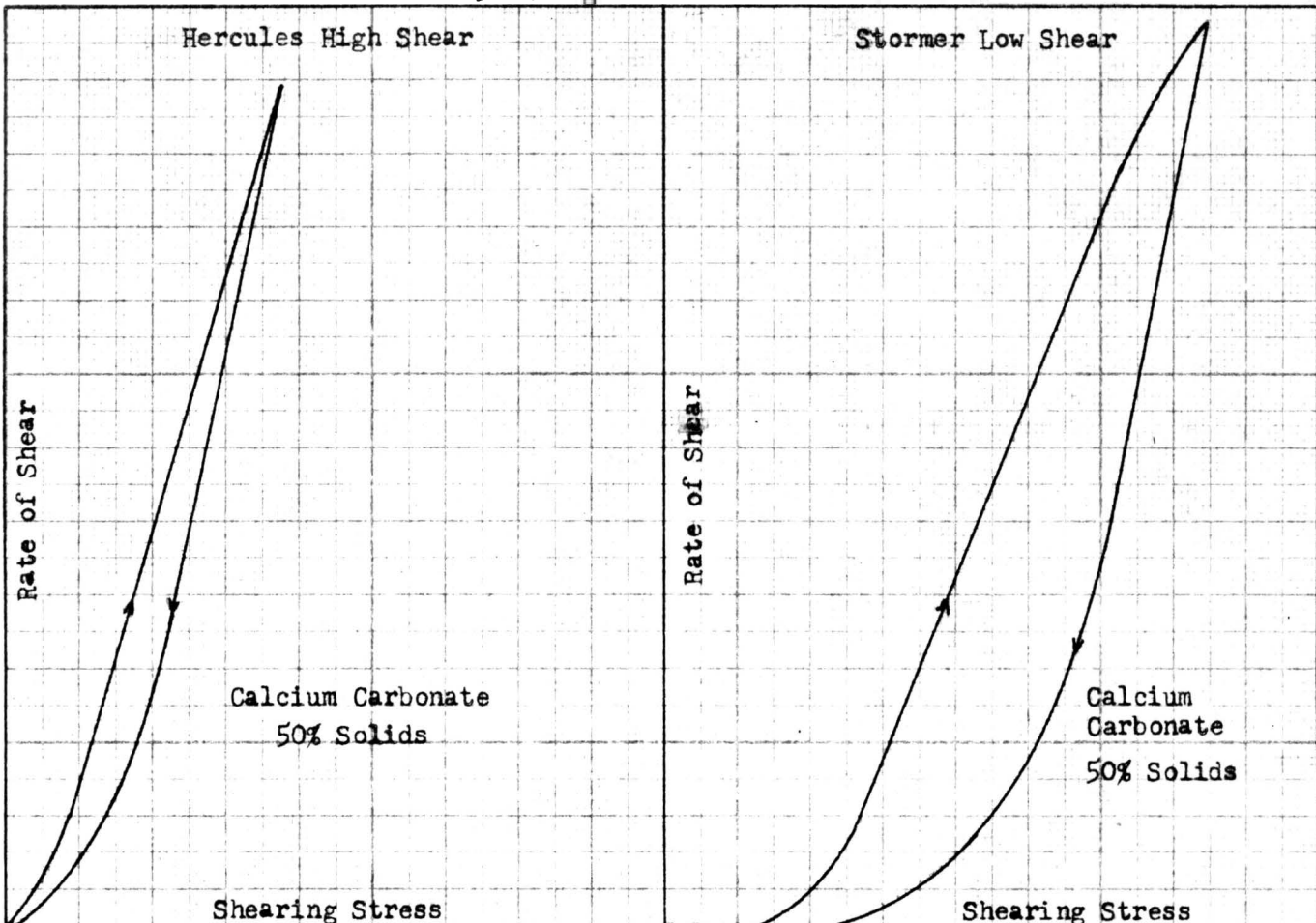
Chart No. 3 Rheograms of Calcium Carbonate
