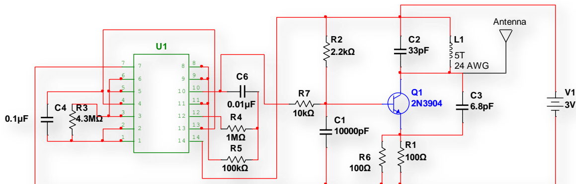
Figure 1. Tracking system circuit diagram.
