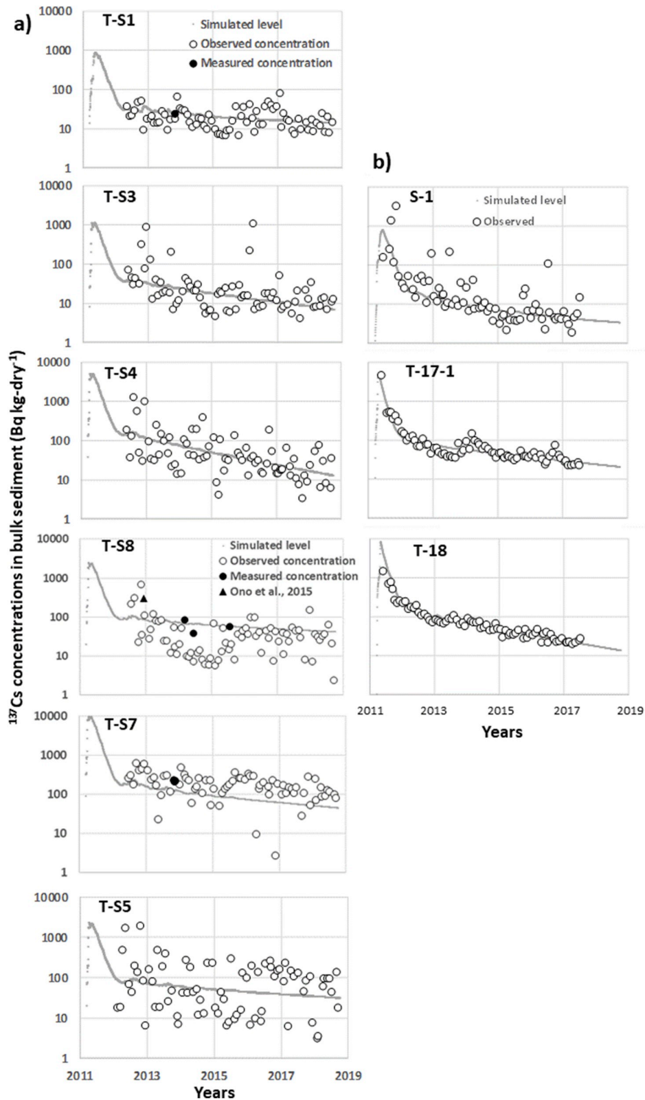
Fig. 4. a) Simulated (gray solid line) and observed ^{137}\text{Cs} concentrations ( \circ ) and the measured concentrations in this study ( \bullet ) over time in bulk surface sediment at TEPCO monitoring stations (T-S1 to T-S8) during 2011–2019. The reported concentration ( \blacktriangle ) is also shown. b) Simulated (gray solid line) and observed ^{137}\text{Cs} concentrations ( \circ ) over time in bulk surface sediment at Fukushima Prefecture monitoring stations (S-1, T-17-1, T-18) during 2011–2018.
